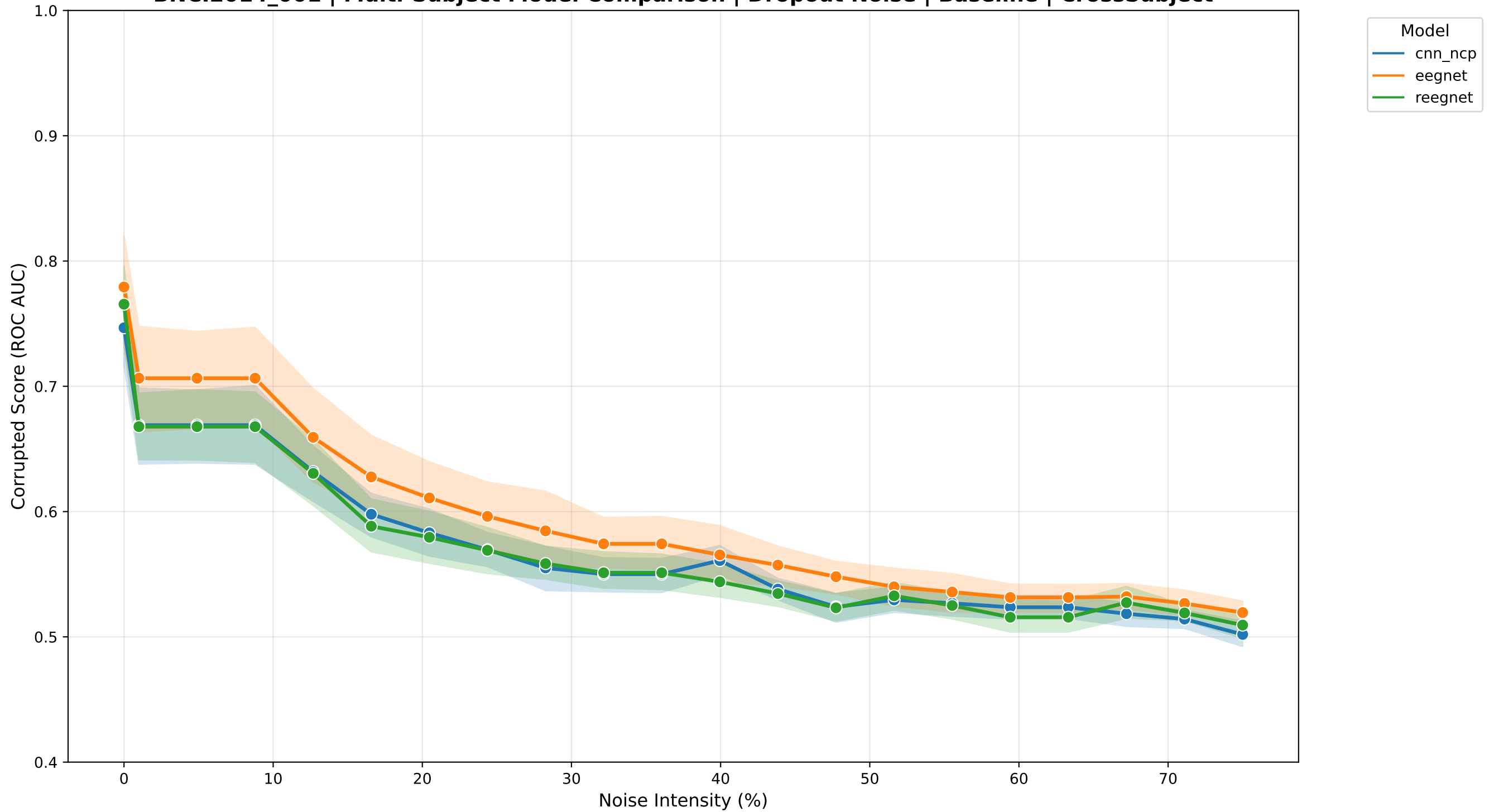
BNCI2014_001 | Multi-Subject Model Comparison | Dropout Noise | Baseline | CrossSubject
