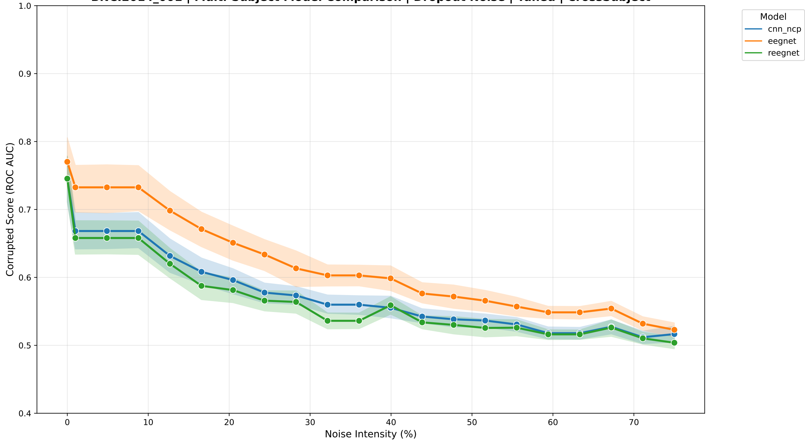
BNCI2014_001 | Multi-Subject Model Comparison | Dropout Noise | Tuned | CrossSubject
