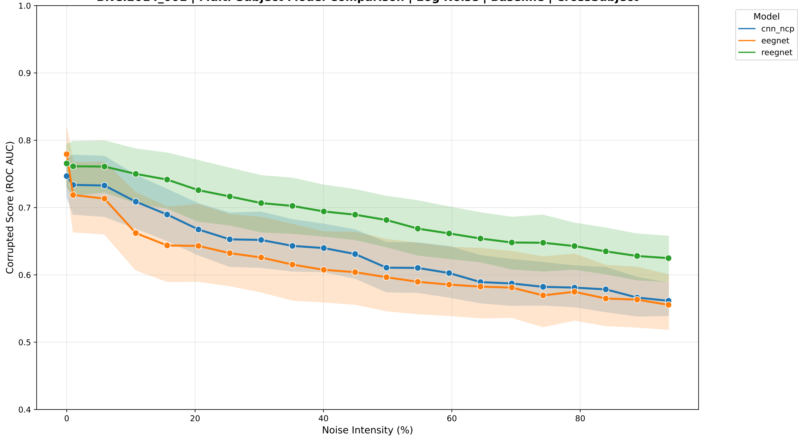
BNCI2014_001 | Multi-Subject Model Comparison | Eog Noise | Baseline | CrossSubject
