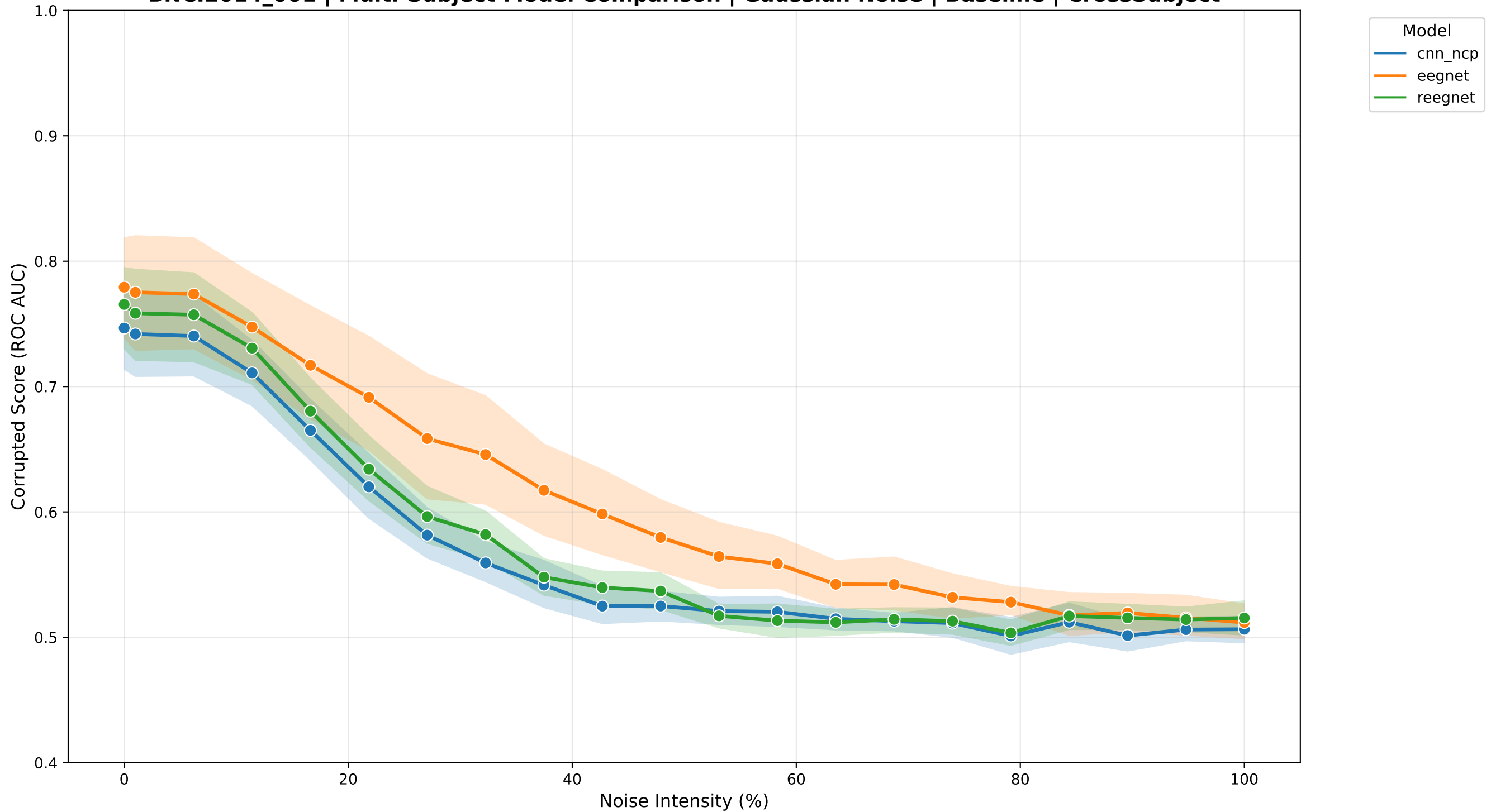
BNCI2014_001 | Multi-Subject Model Comparison | Gaussian Noise | Baseline | CrossSubject
