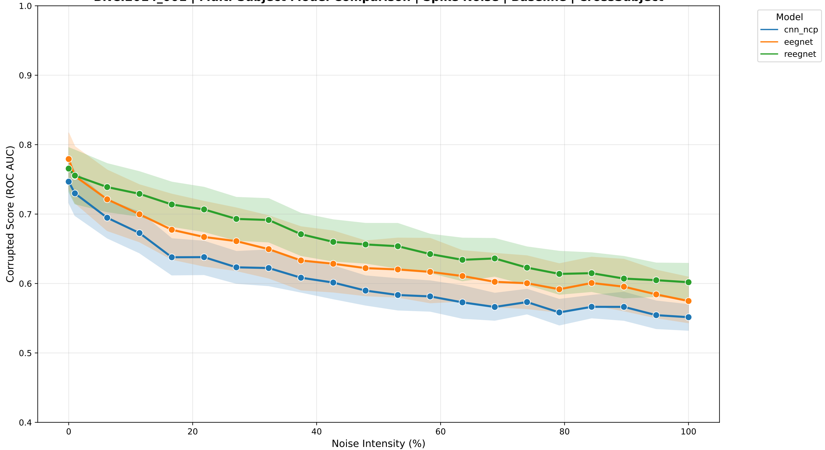
BNCI2014_001 | Multi-Subject Model Comparison | Spike Noise | Baseline | CrossSubject
