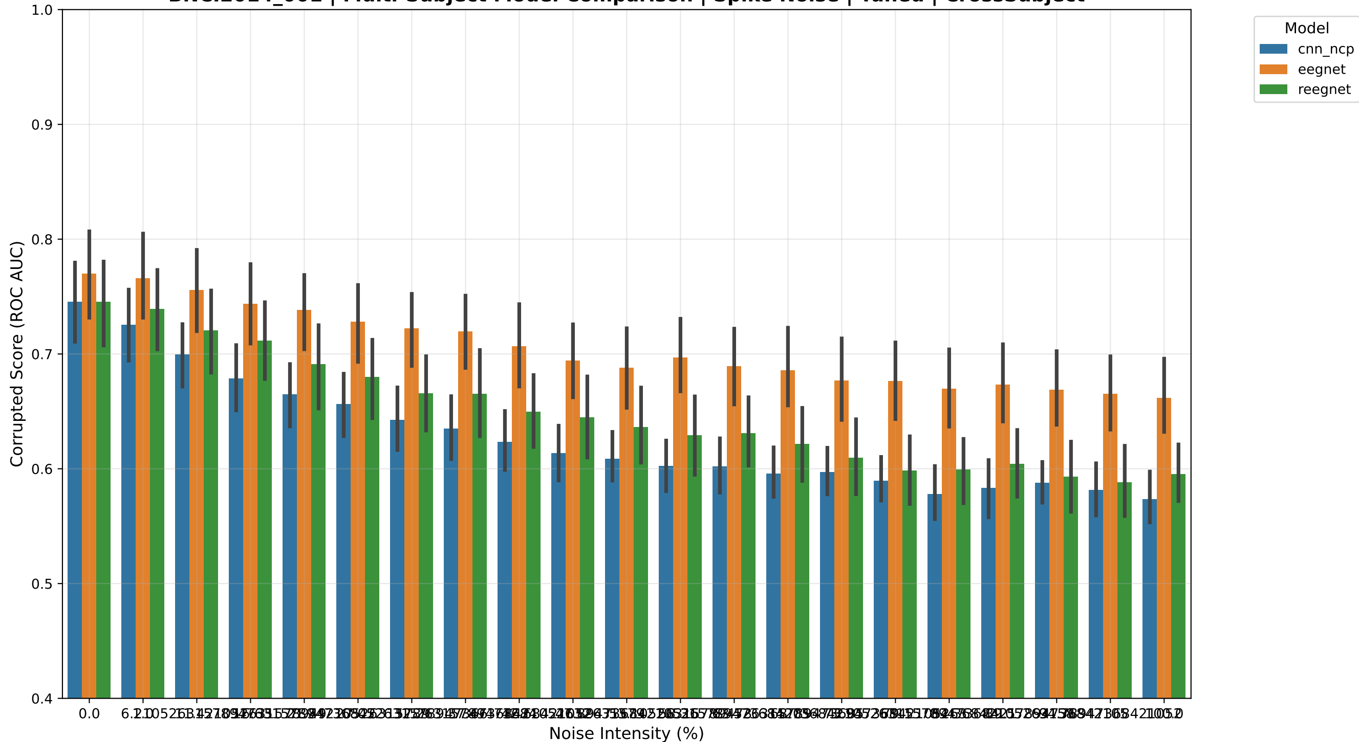
BNCI2014_001 | Multi-Subject Model Comparison | Spike Noise | Tuned | CrossSubject
