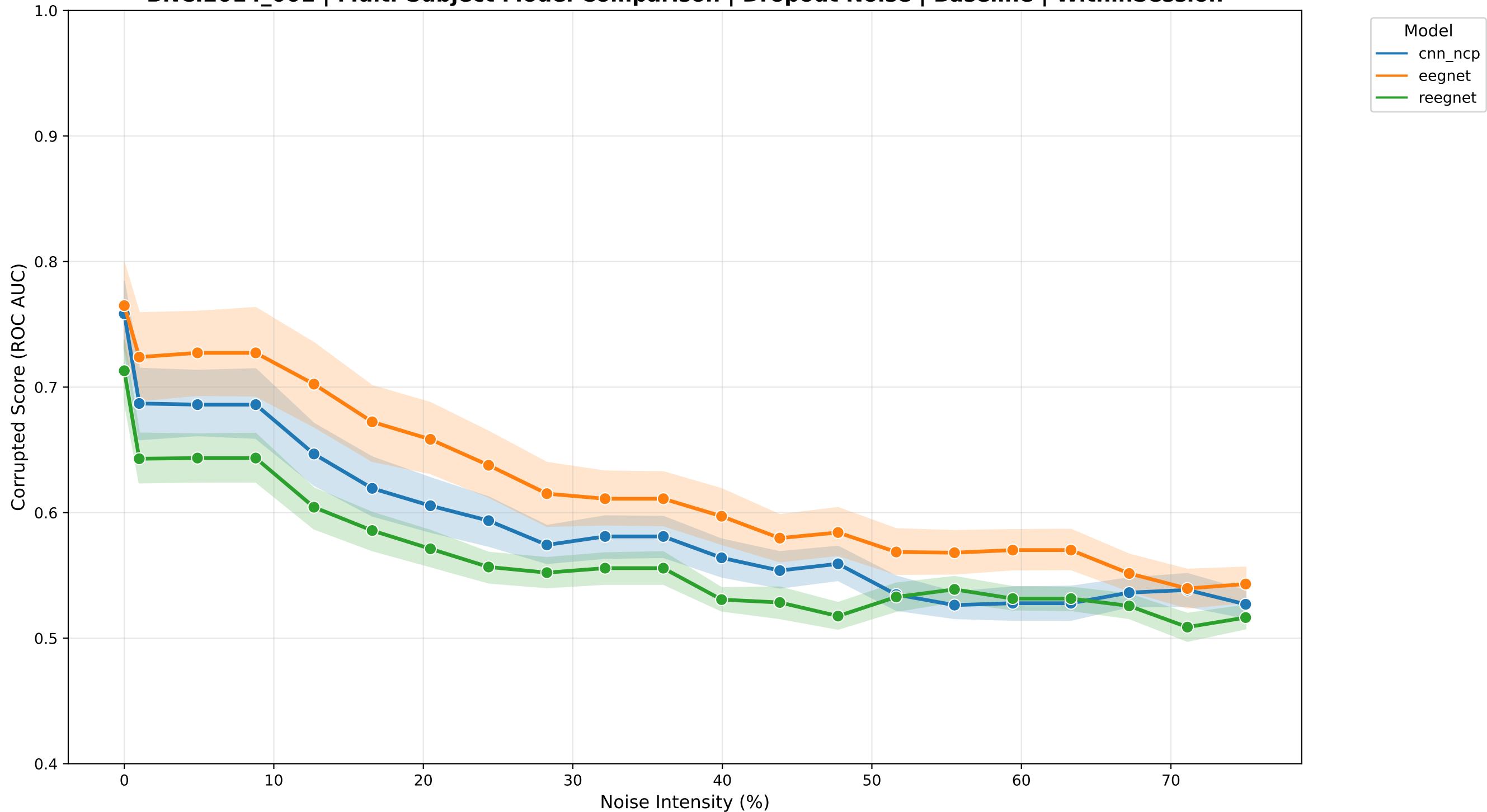
BNCI2014_001 | Multi-Subject Model Comparison | Dropout Noise | Baseline | WithinSession
