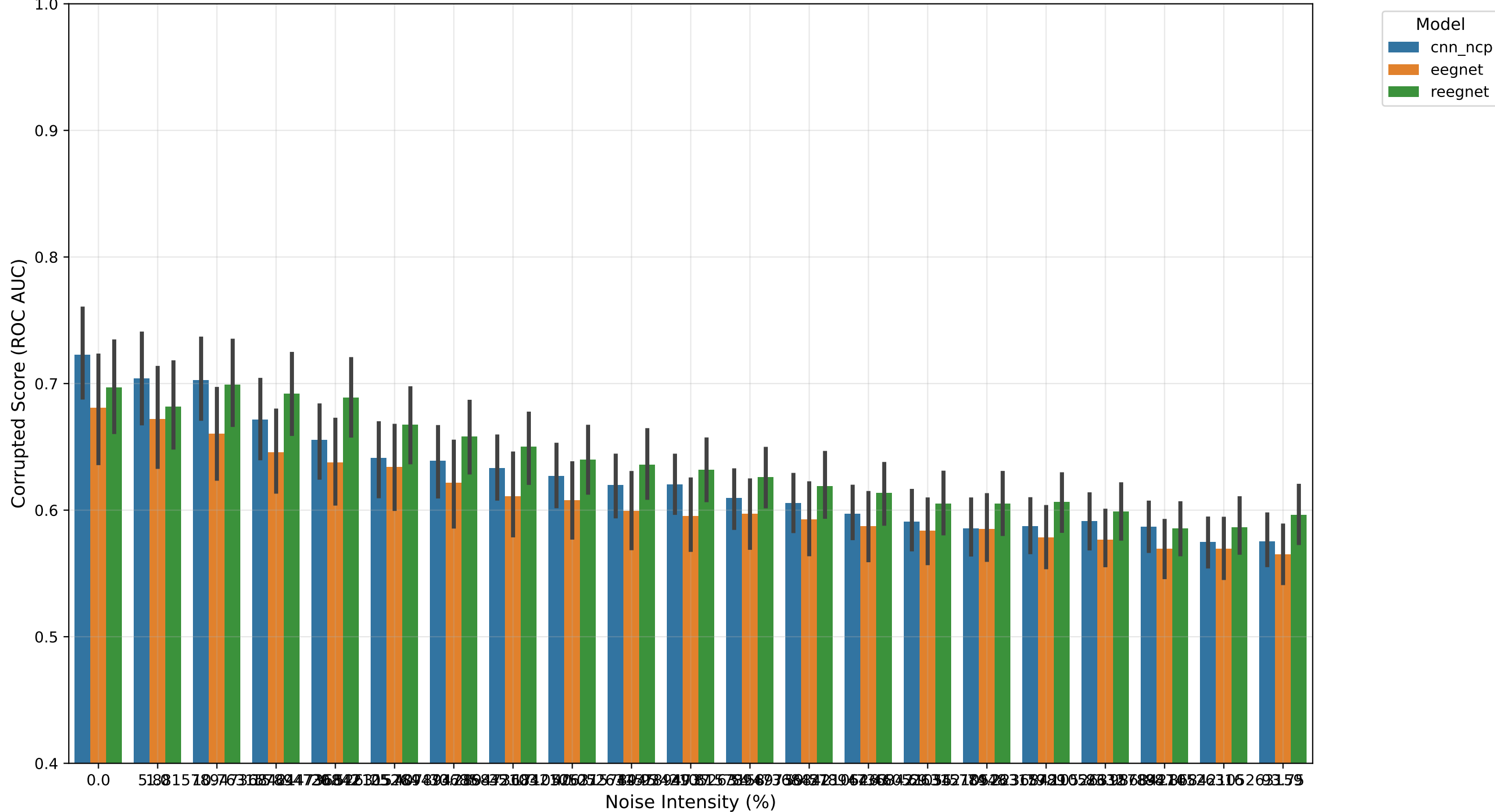
BNCI2014_001 | Multi-Subject Model Comparison | Eog Noise | Tuned | WithinSession
