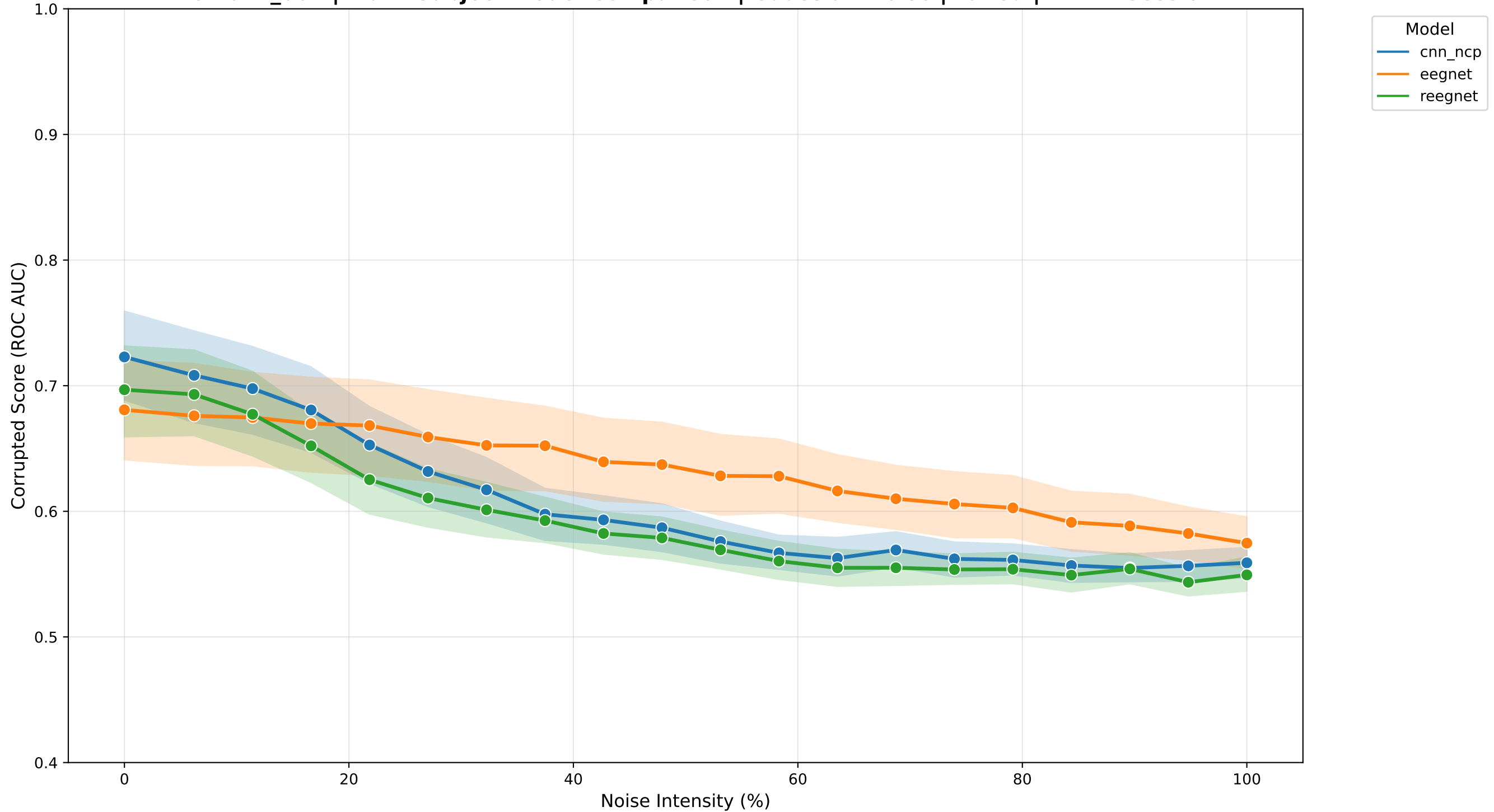
BNCI2014_001 | Multi-Subject Model Comparison | Gaussian Noise | Tuned | WithinSession
