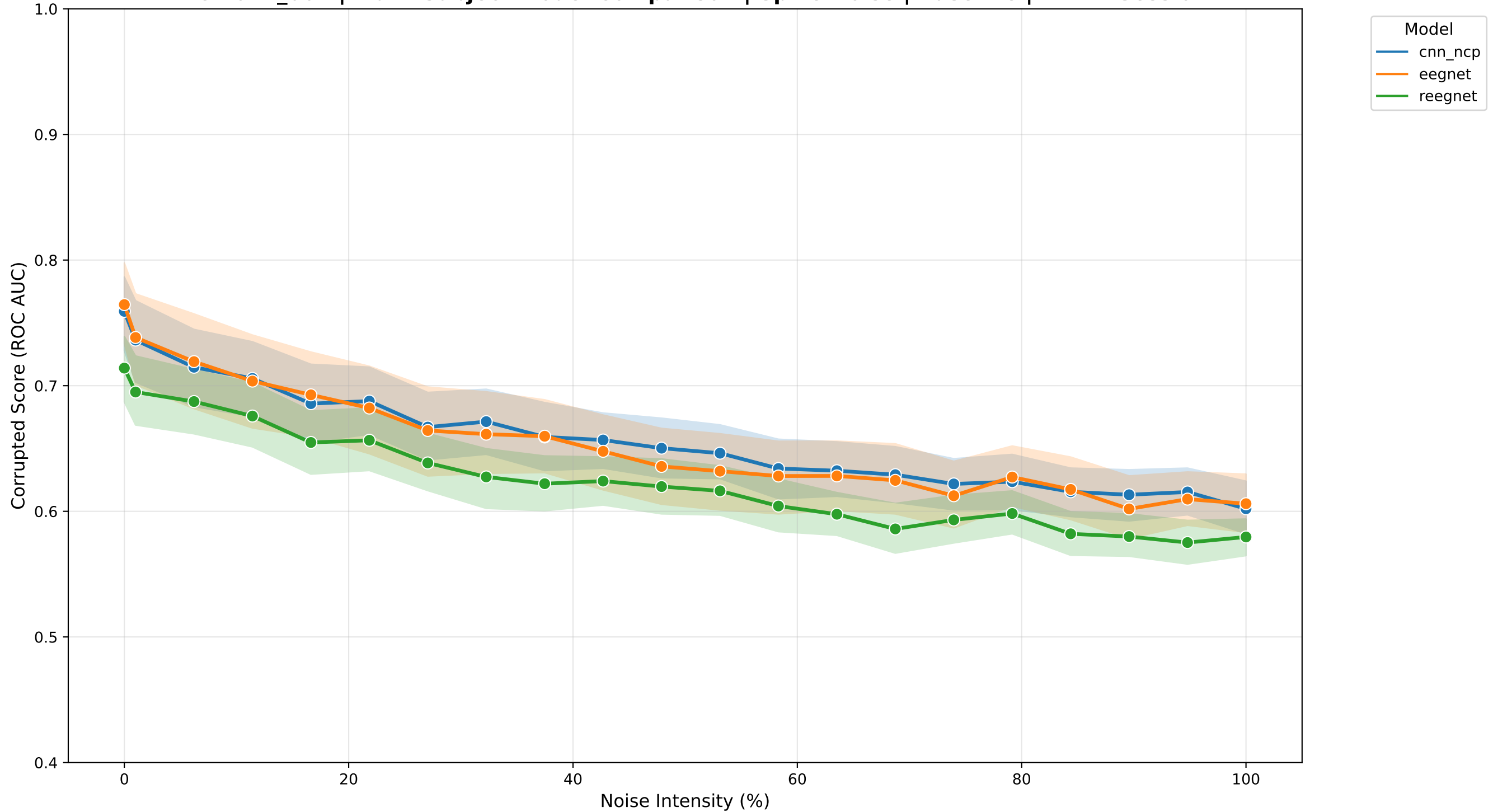
BNCI2014_001 | Multi-Subject Model Comparison | Spike Noise | Baseline | WithinSession
