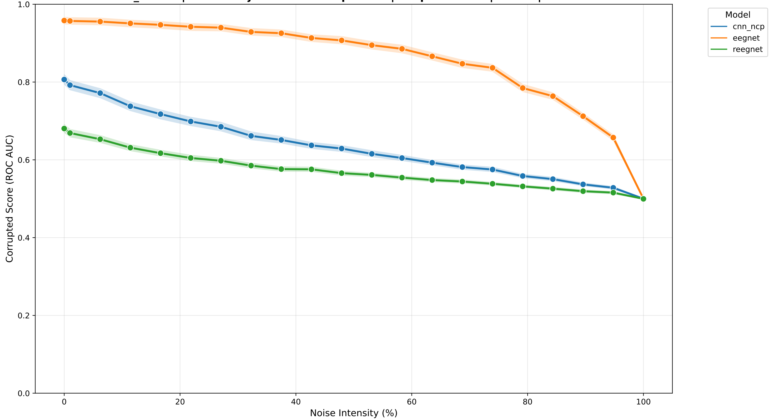
Lee2019_SSVEP | Multi-Subject Model Comparison | Dropout Noise | Tuned | CrossSession
