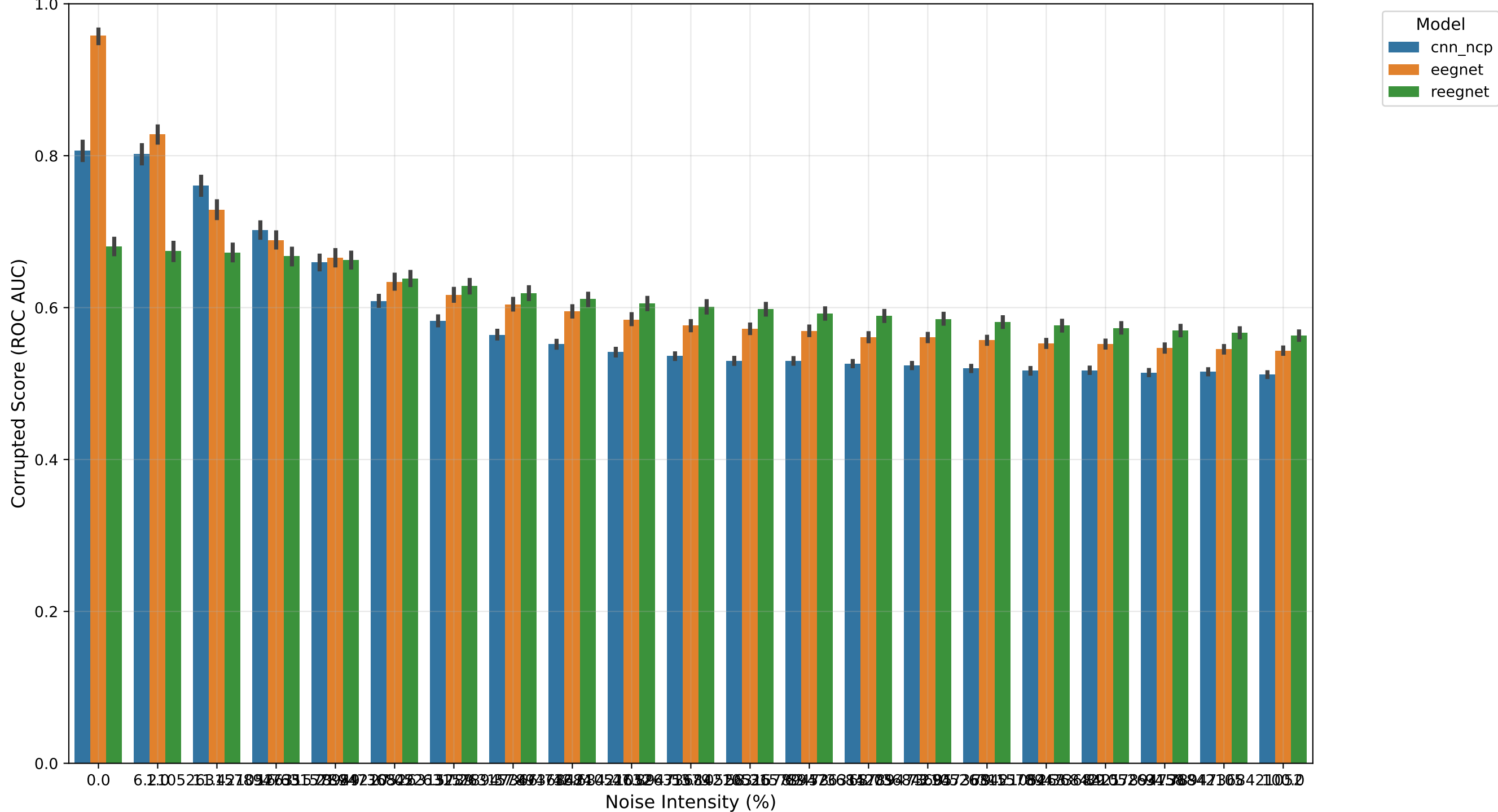
Lee2019_SSVEP | Multi-Subject Model Comparison | Eog Noise | Tuned | CrossSession
