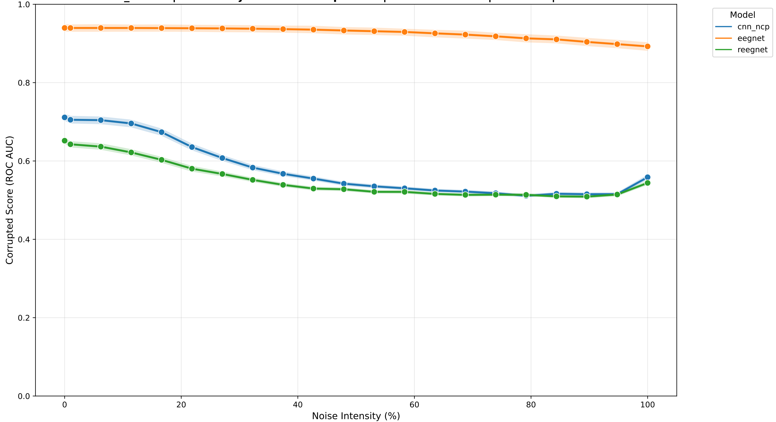
Lee2019_SSVEP | Multi-Subject Model Comparison | Gaussian Noise | Baseline | CrossSession
