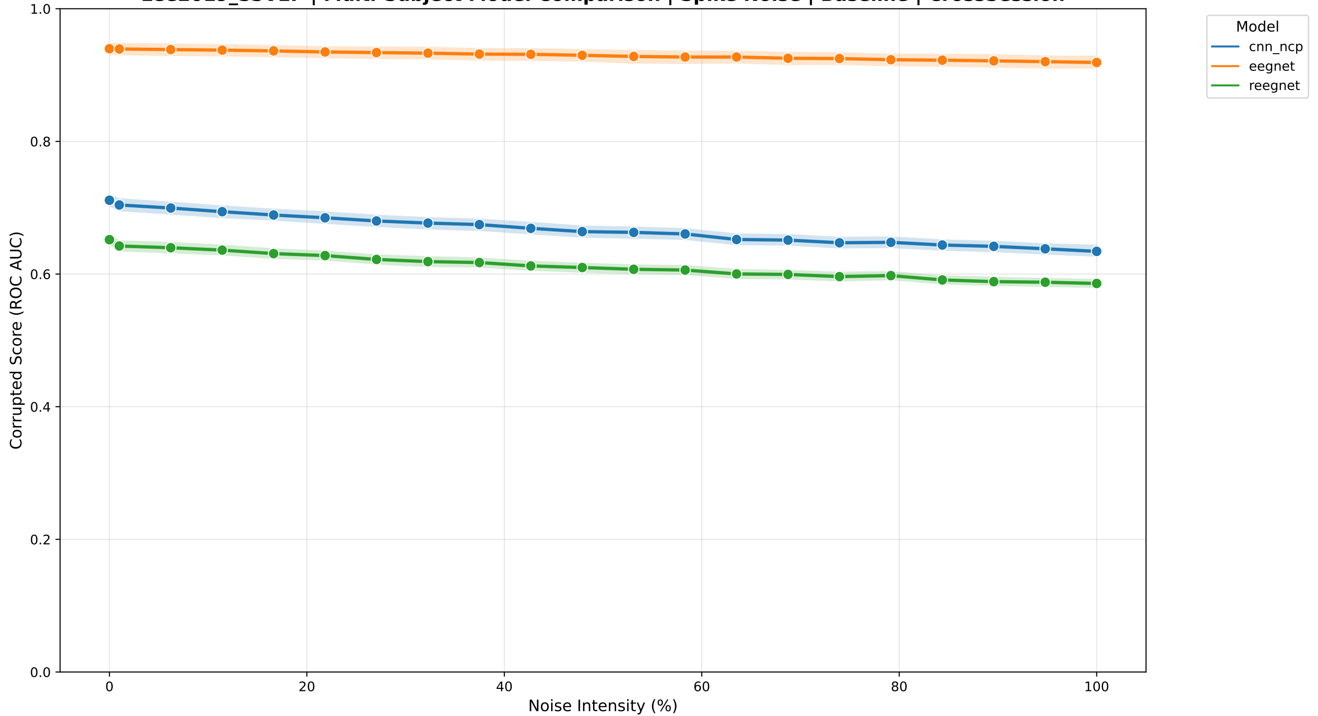
Lee2019_SSVEP | Multi-Subject Model Comparison | Spike Noise | Baseline | CrossSession
