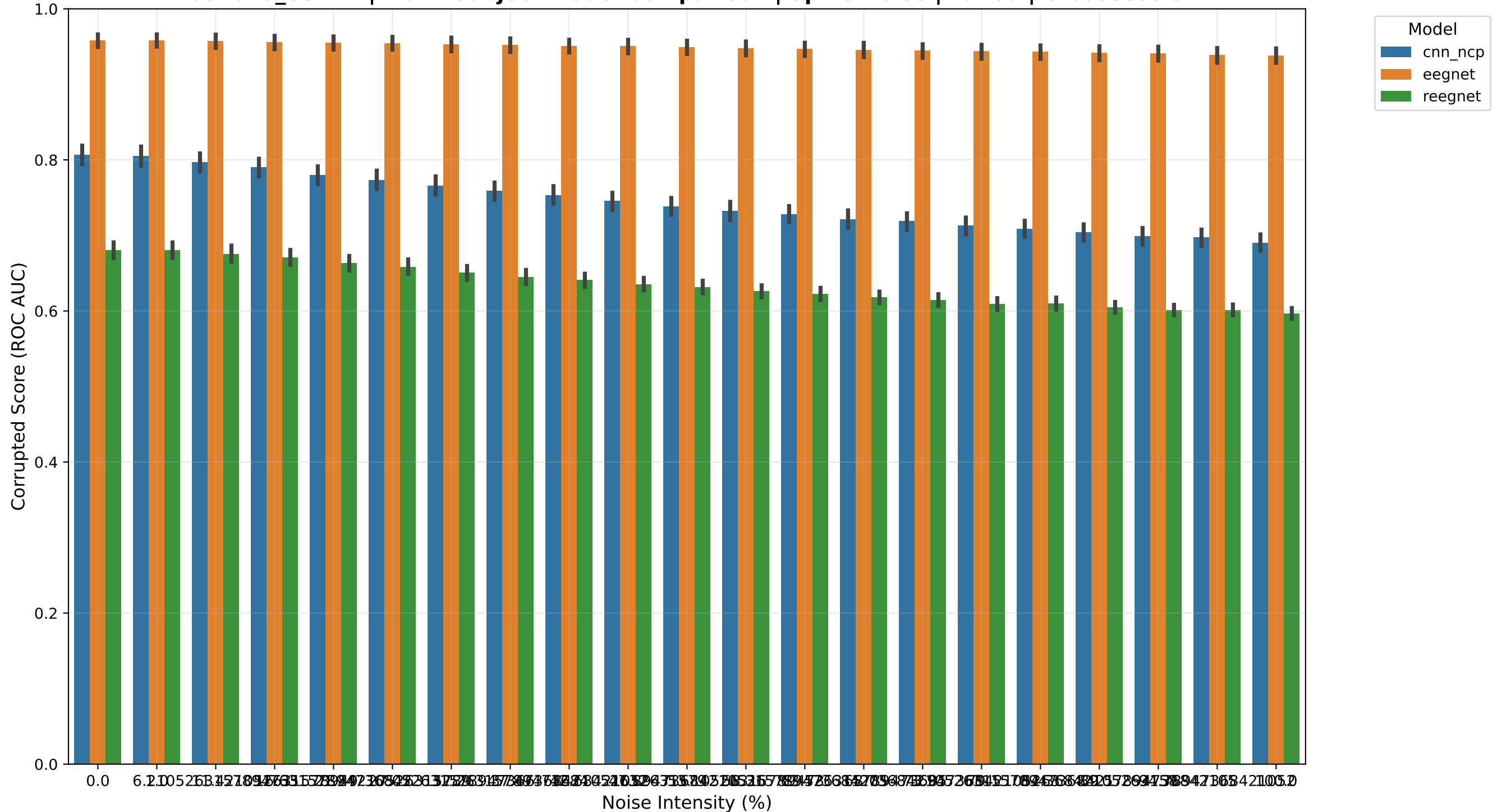
Lee2019_SSVEP | Multi-Subject Model Comparison | Spike Noise | Tuned | CrossSession
