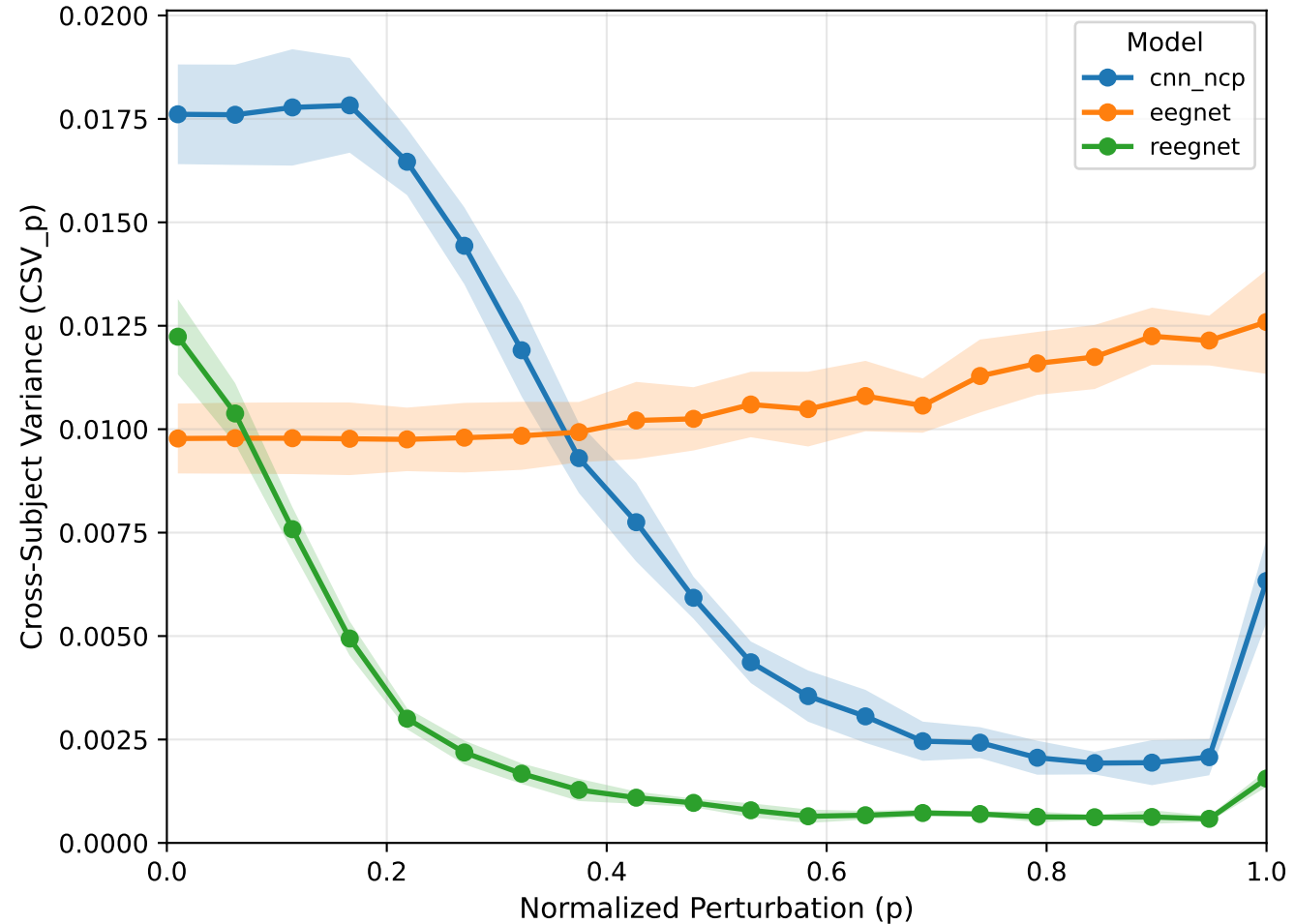
Tuned
