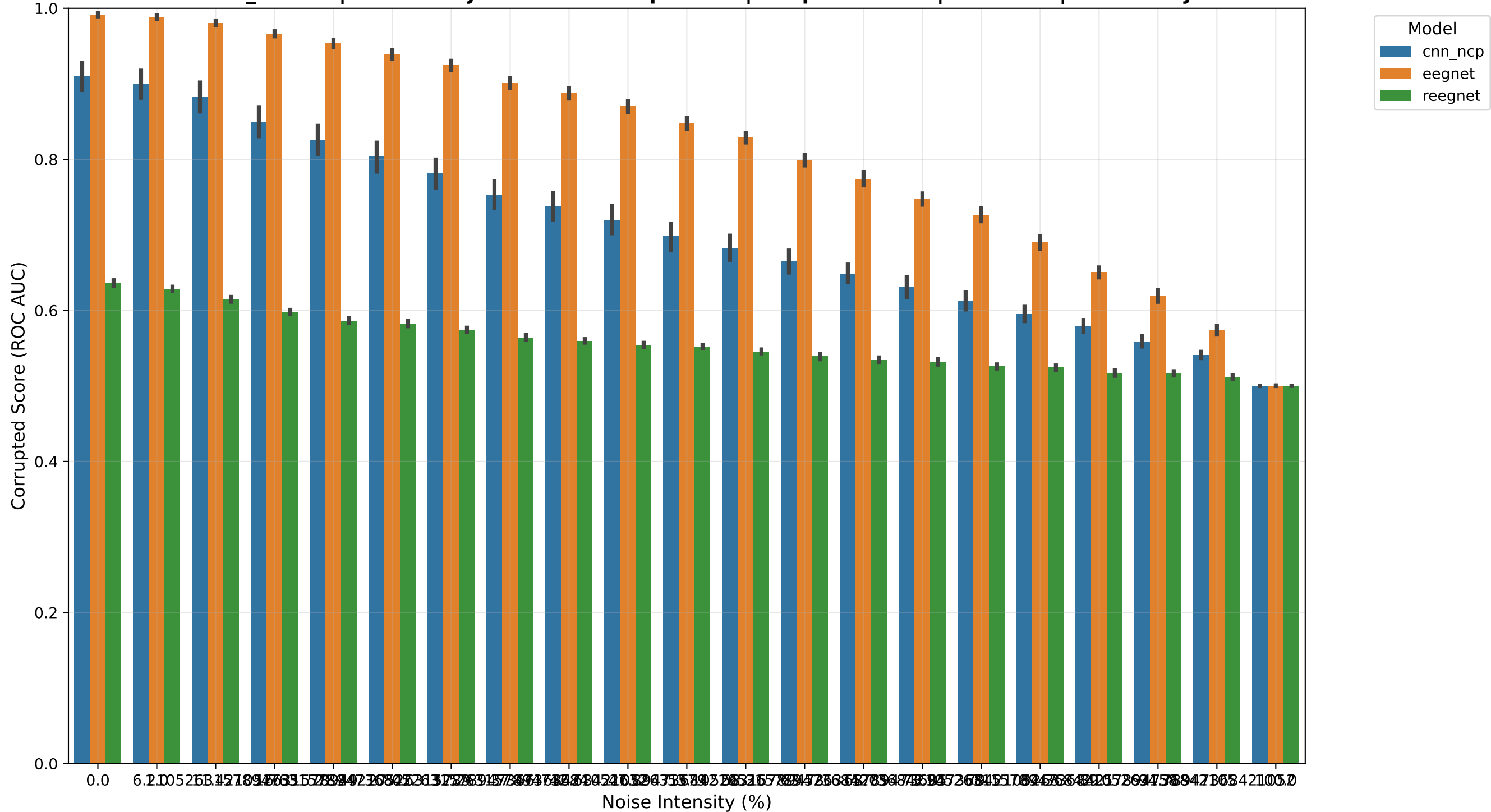
Lee2019_SSVEP | Multi-Subject Model Comparison | Dropout Noise | Baseline | CrossSubject
