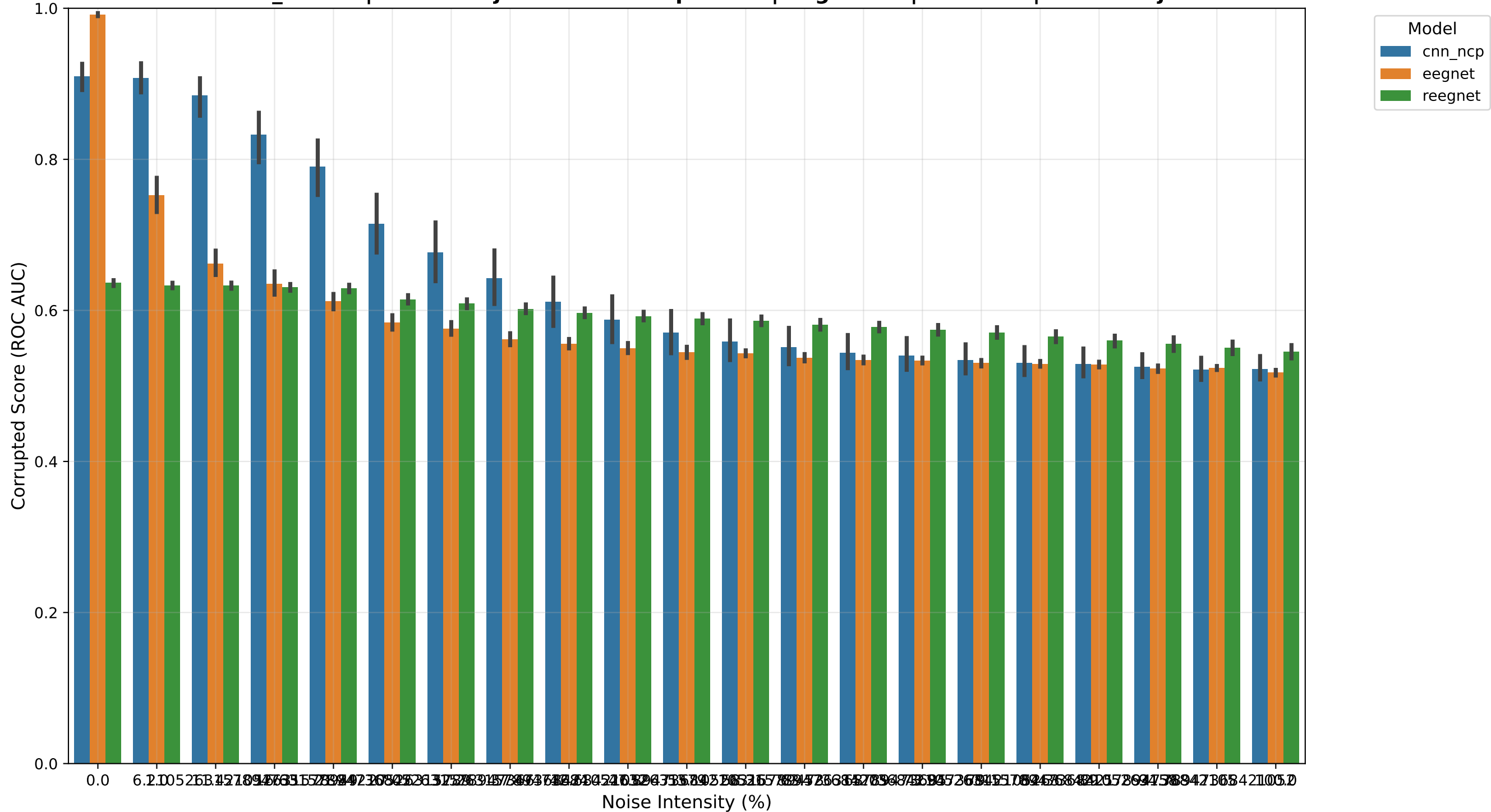
Lee2019_SSVEP | Multi-Subject Model Comparison | Eog Noise | Baseline | CrossSubject
