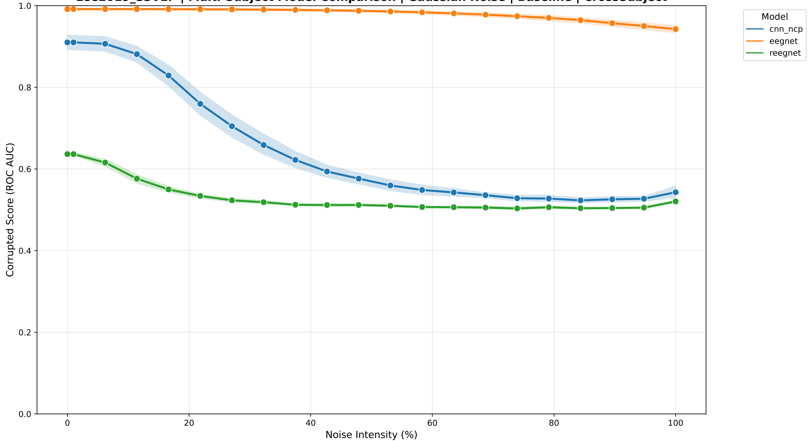
Lee2019_SSVEP | Multi-Subject Model Comparison | Gaussian Noise | Baseline | CrossSubject
