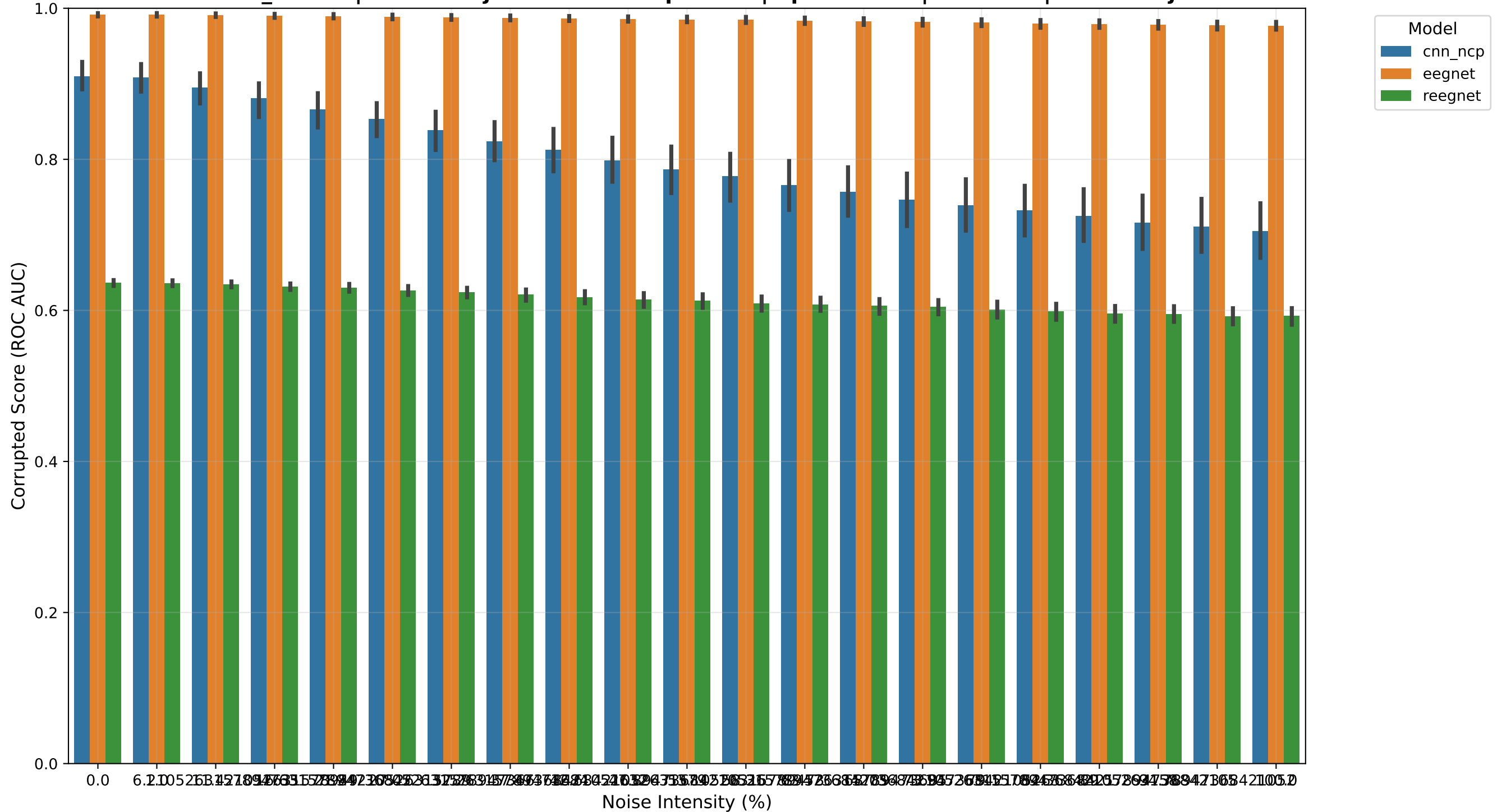
Lee2019_SSVEP | Multi-Subject Model Comparison | Spike Noise | Baseline | CrossSubject
