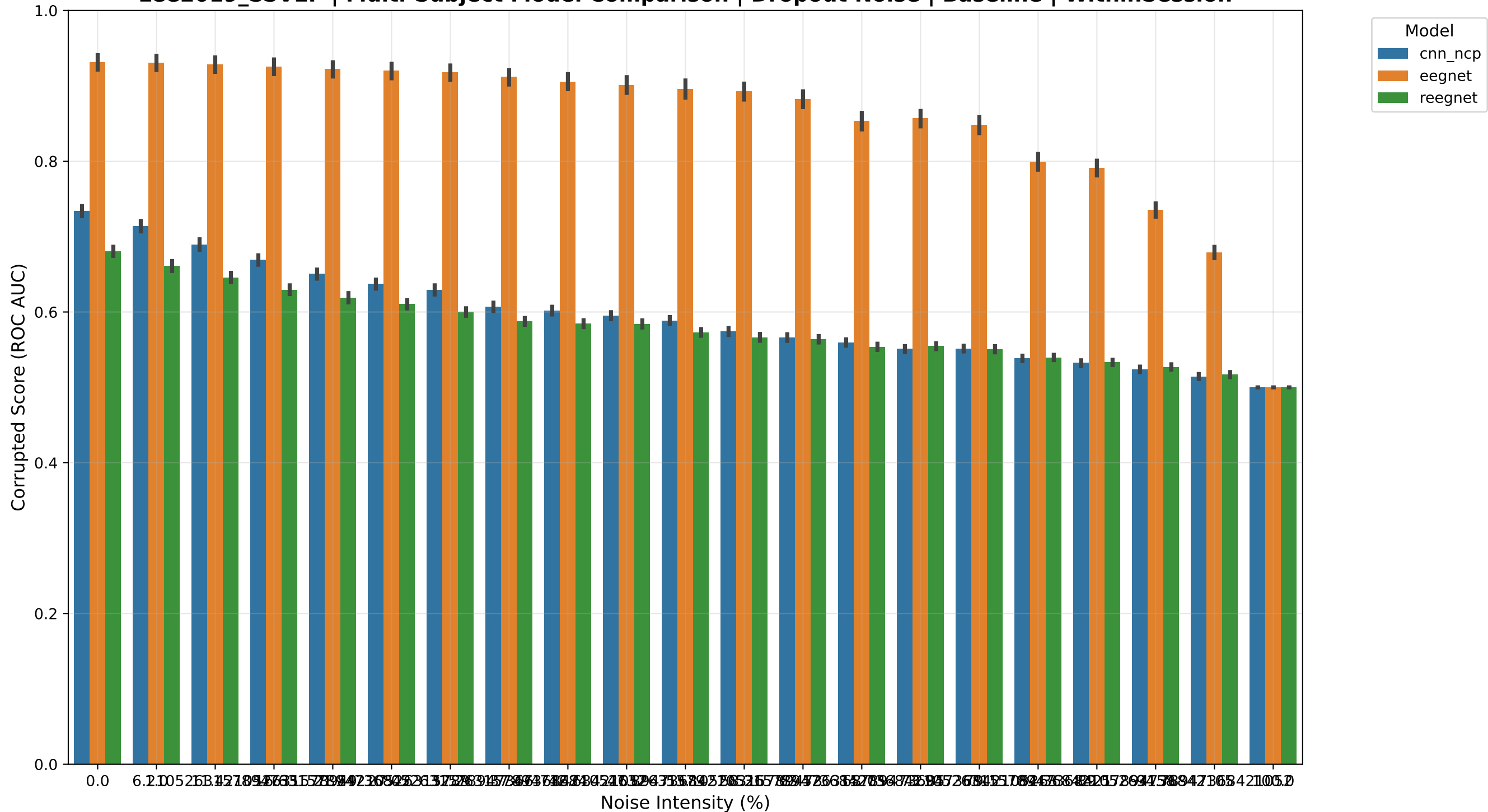
Lee2019_SSVEP | Multi-Subject Model Comparison | Dropout Noise | Baseline | WithinSession
