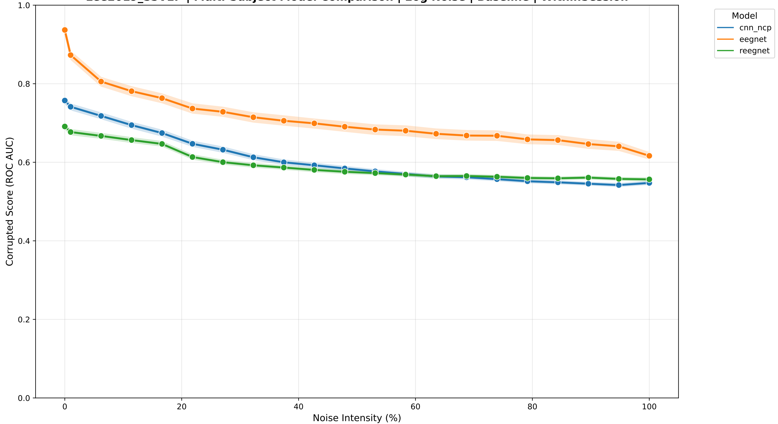
Lee2019_SSVEP | Multi-Subject Model Comparison | Eog Noise | Baseline | WithinSession
