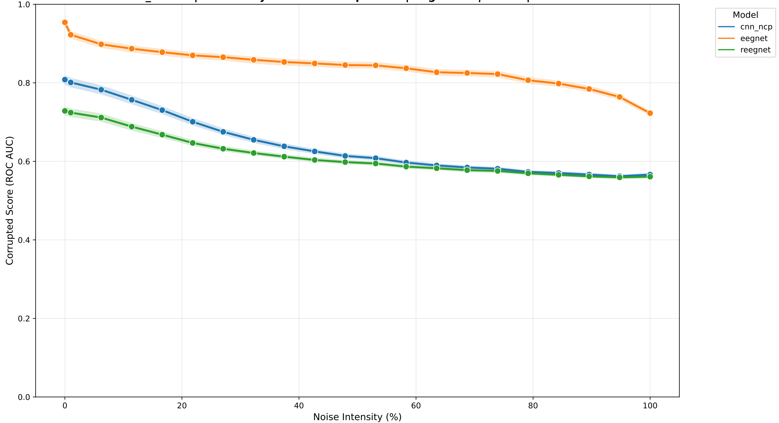
Lee2019_SSVEP | Multi-Subject Model Comparison | Eog Noise | Tuned | WithinSession
