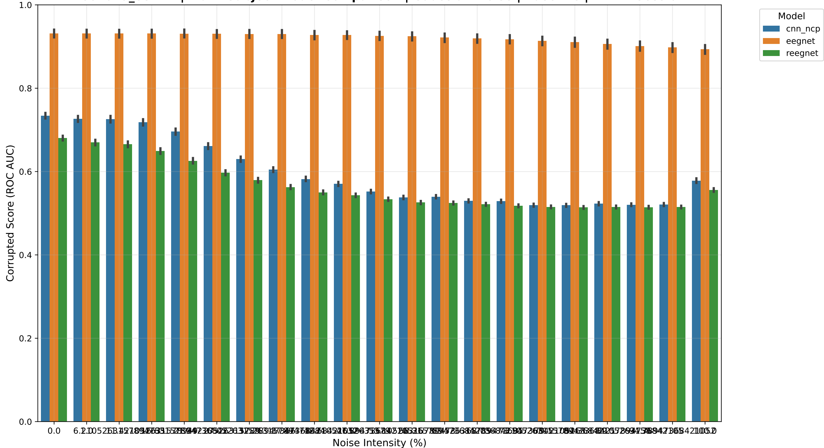
Lee2019_SSVEP | Multi-Subject Model Comparison | Gaussian Noise | Baseline | WithinSession
