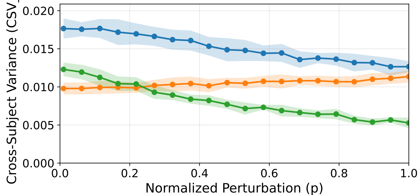
Within-Session | Tuned
