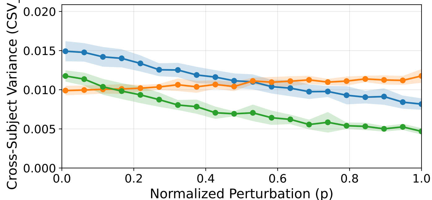
Cross-Subject | Tuned
