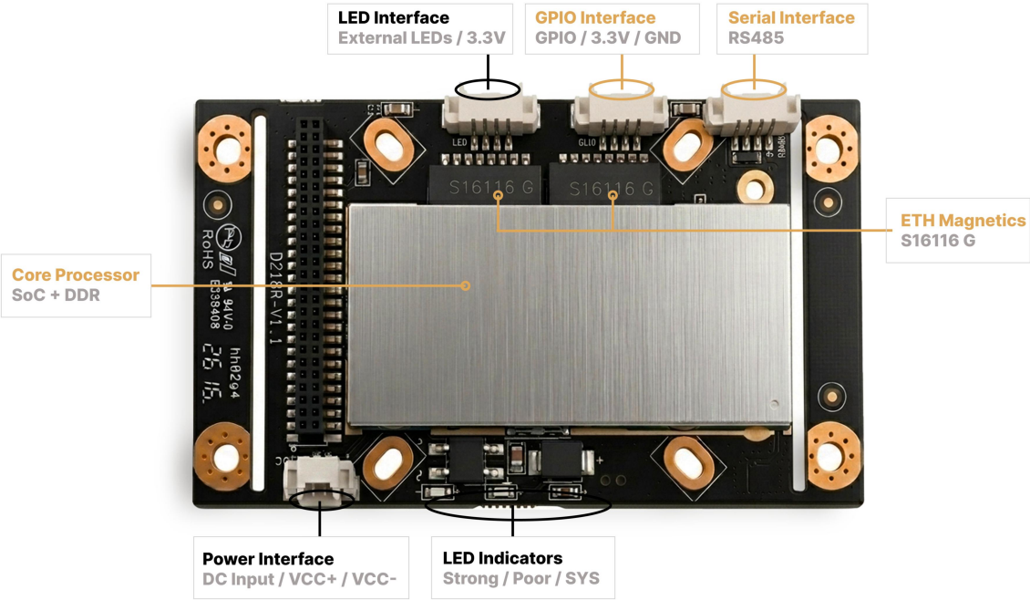
Figure 4. Rear interface and major component layout
