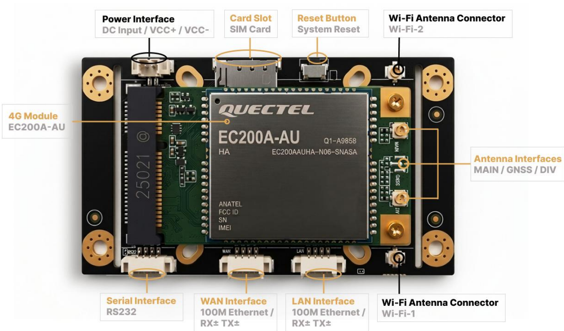
Figure 3. Front interface and major component layout
