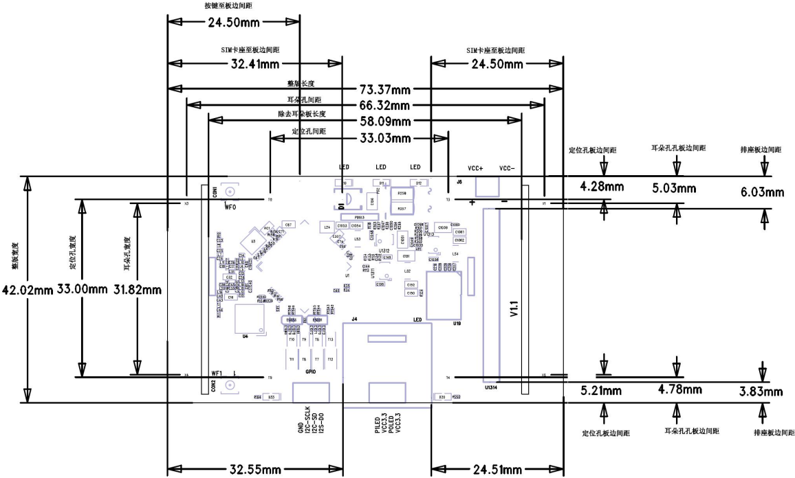
Figure 5. Mechanical dimensions
