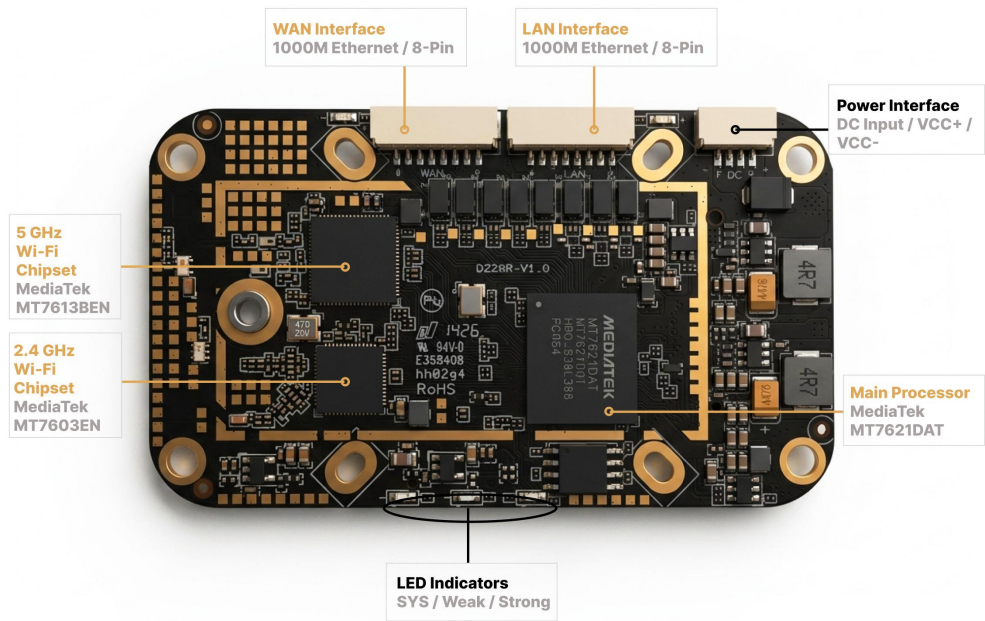
Figure 4. Rear interface and major component layout
