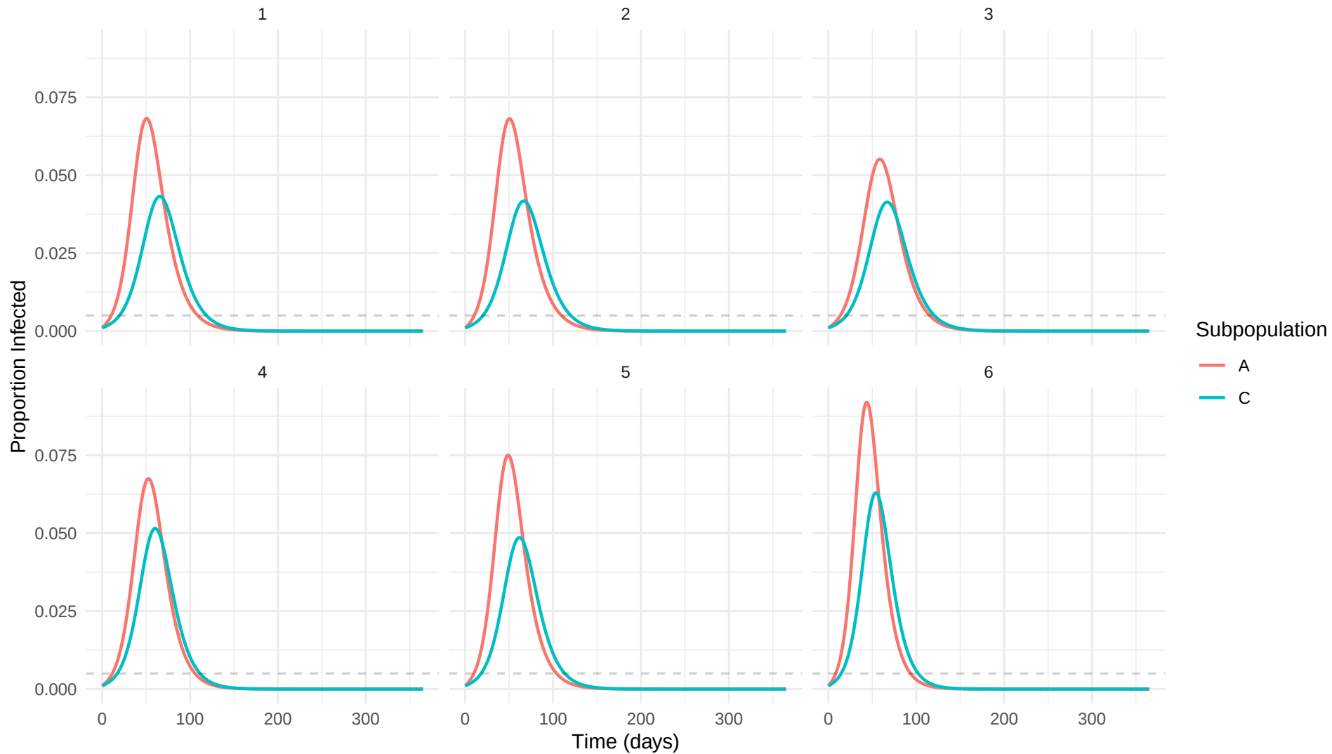
Infection curves: vax_eff_0.2
