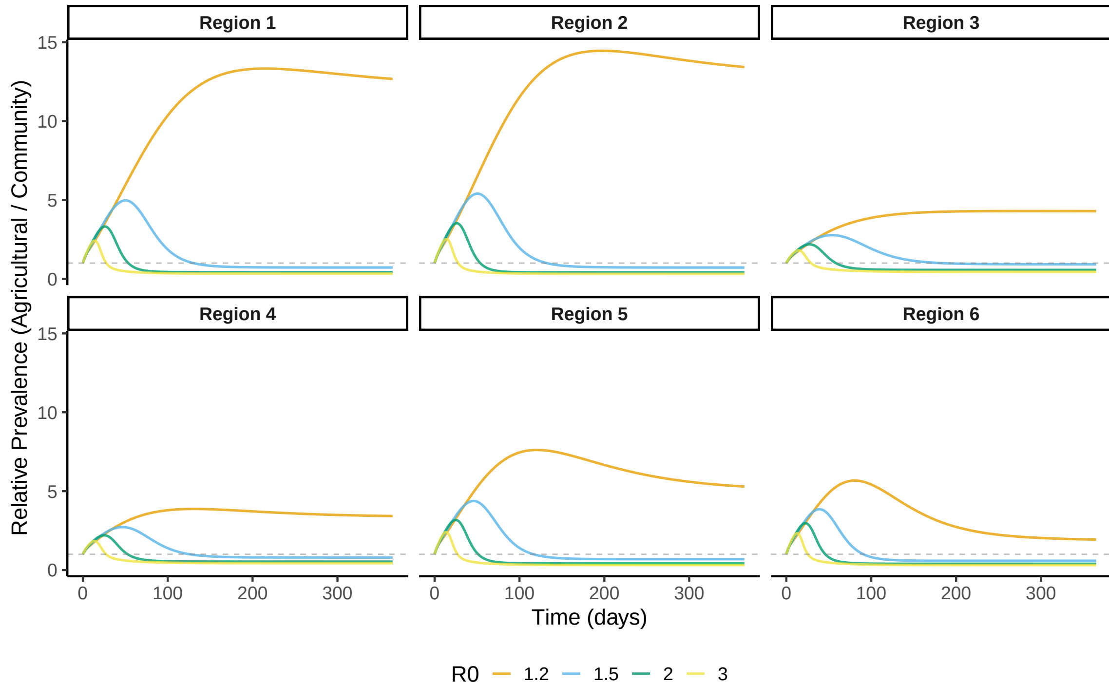
Relative Prevalence by Region – Sensitivity to R0
