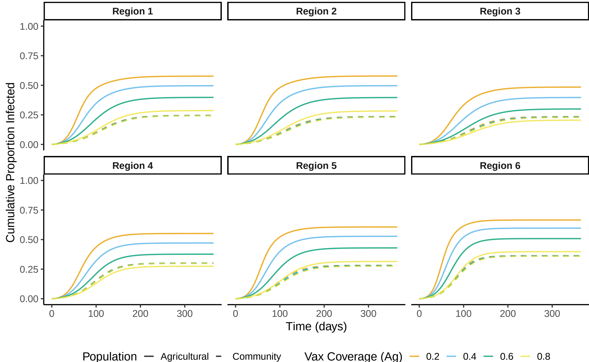
Cumulative Infections by Region – Sensitivity to Vax Coverage (Ag)
