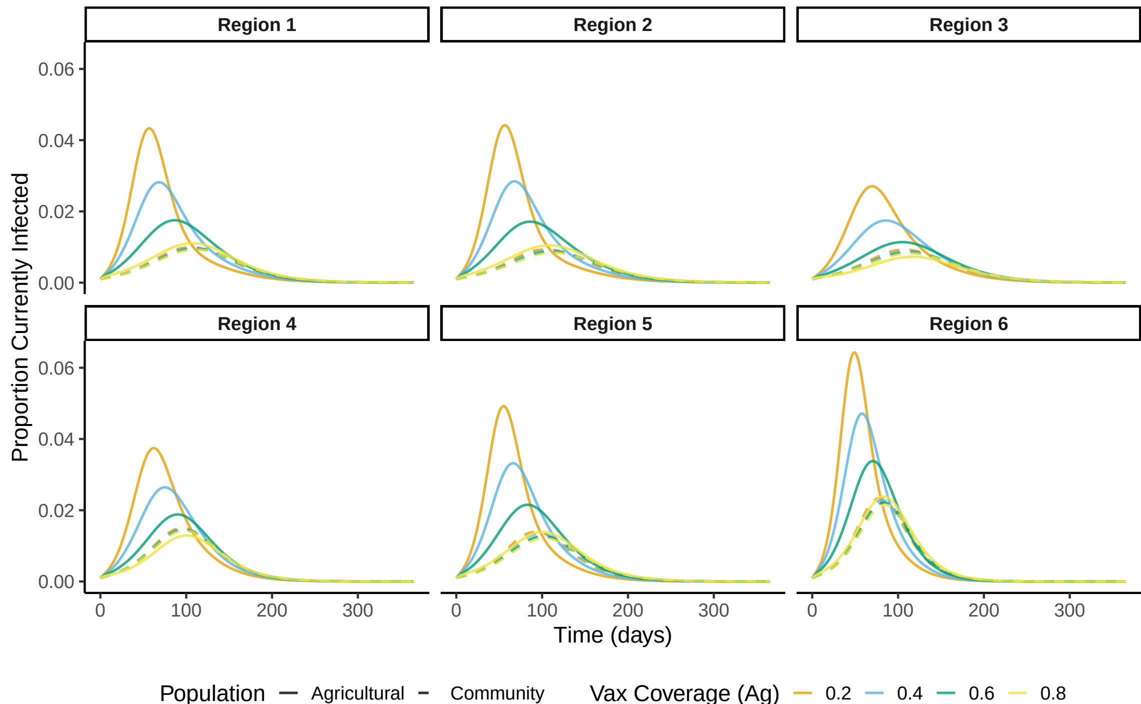
Epidemic Curves by Region – Sensitivity to Vax Coverage (Ag)
