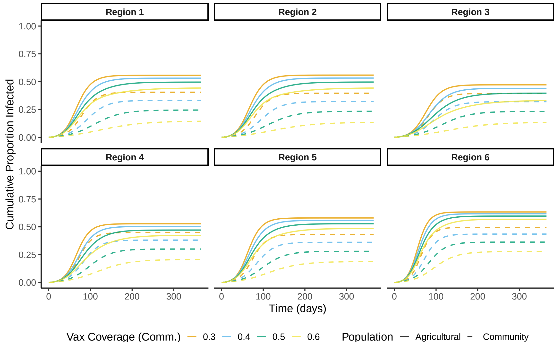
Cumulative Infections by Region – Sensitivity to Vax Coverage (Comm.)
