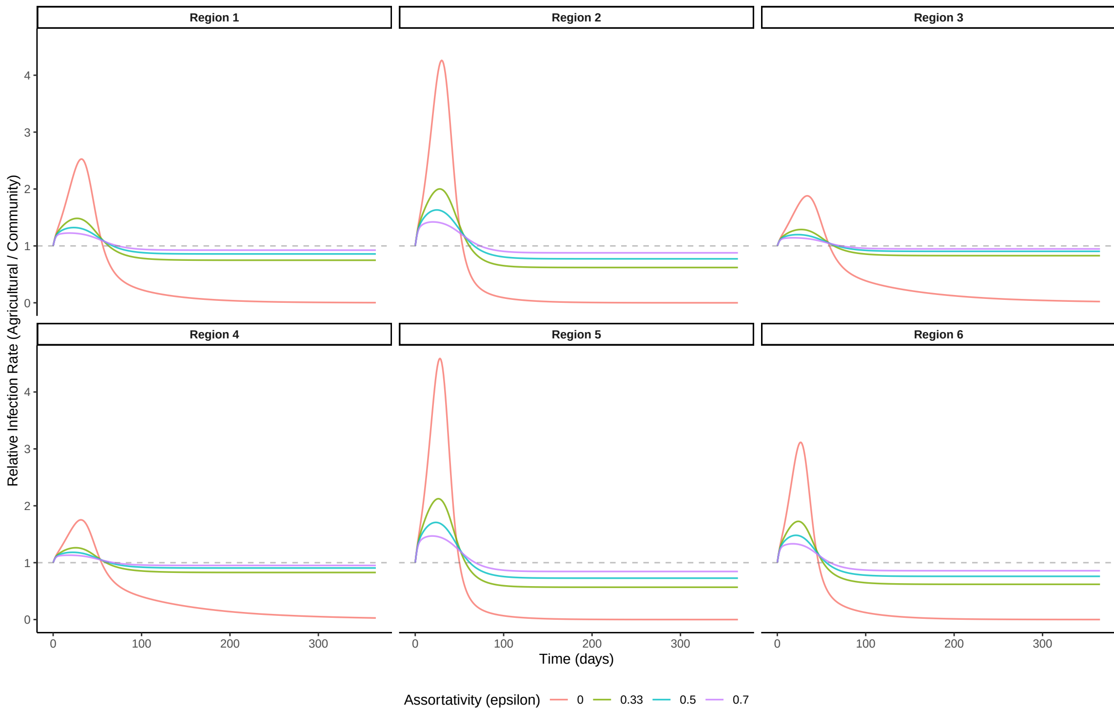
Relative Infection Rate by Region – Sensitivity to Assortativity (epsilon)
