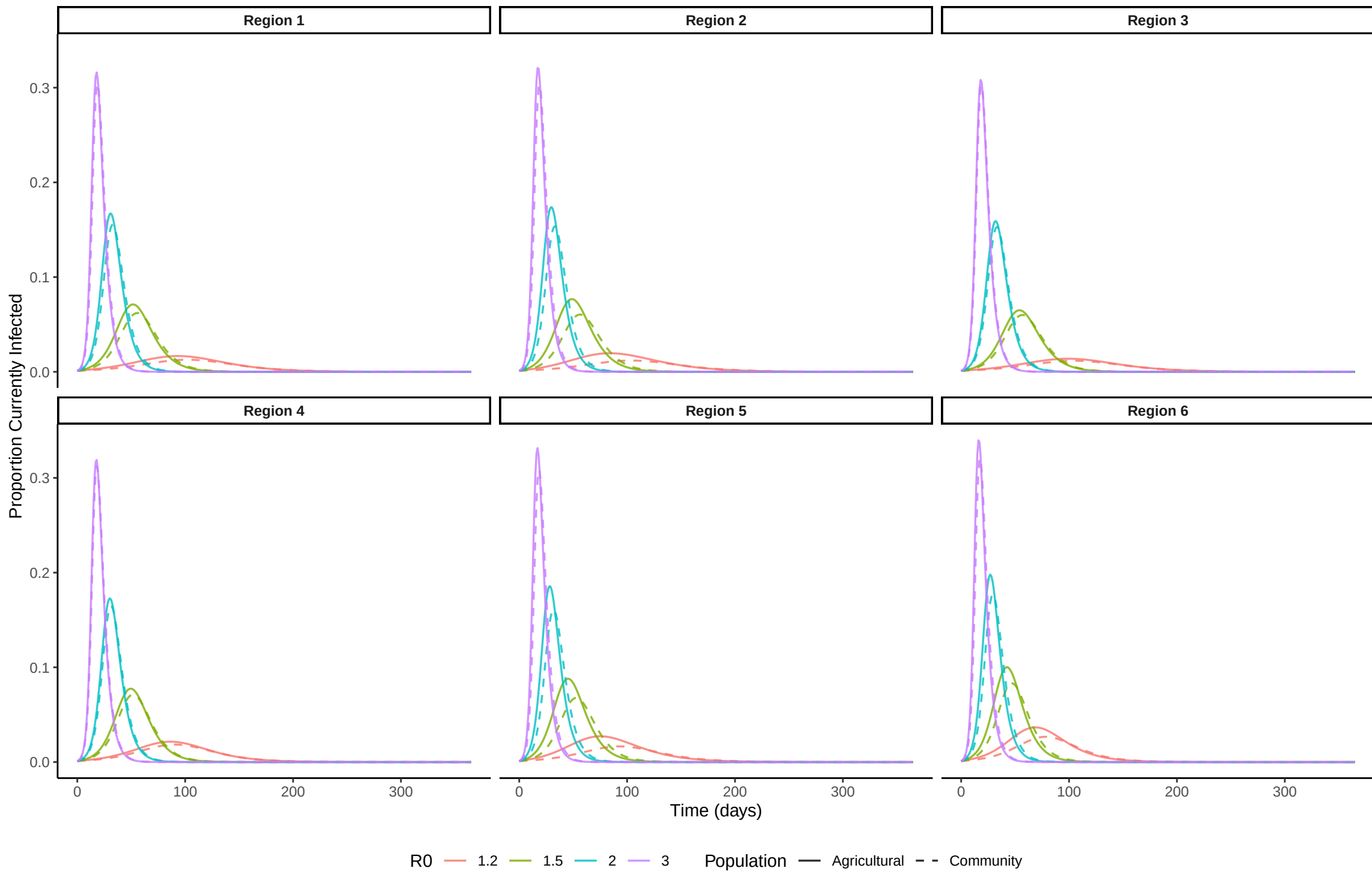
Epidemic Curves by Region – Sensitivity to R0
