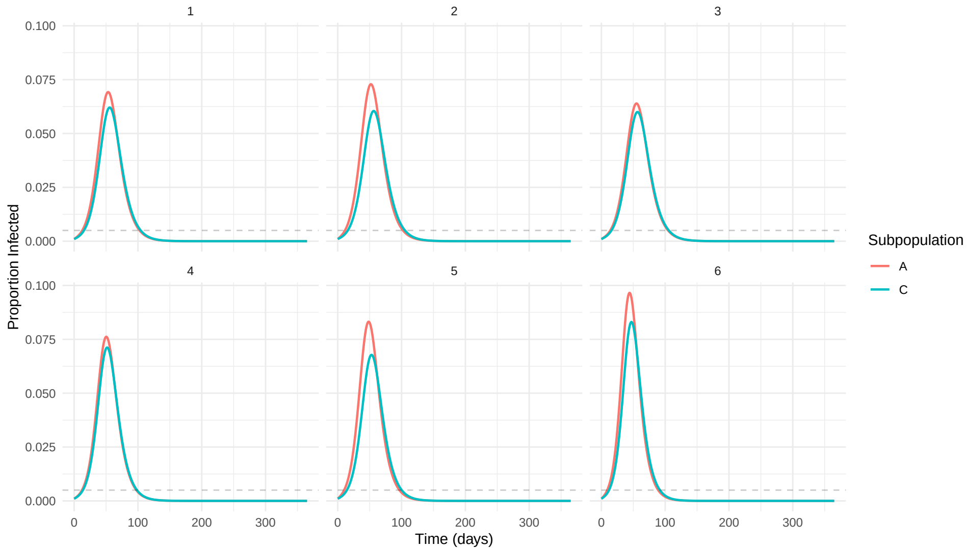
Infection curves: eps_0.5
