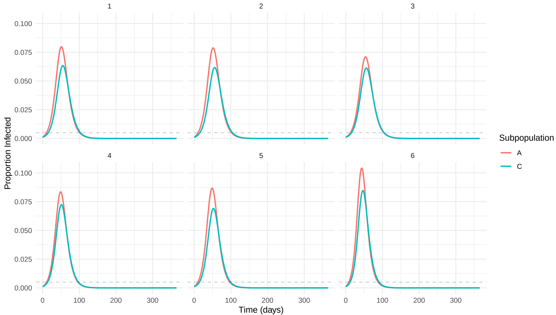
Infection curves: \text{eps\_}0.6667
