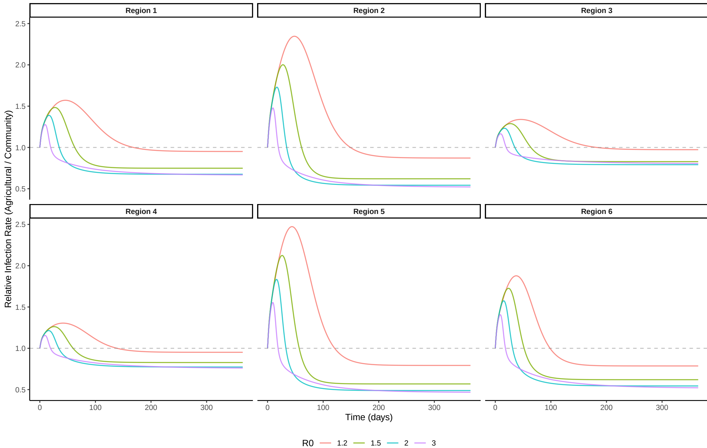
Relative Infection Rate by Region – Sensitivity to R0
