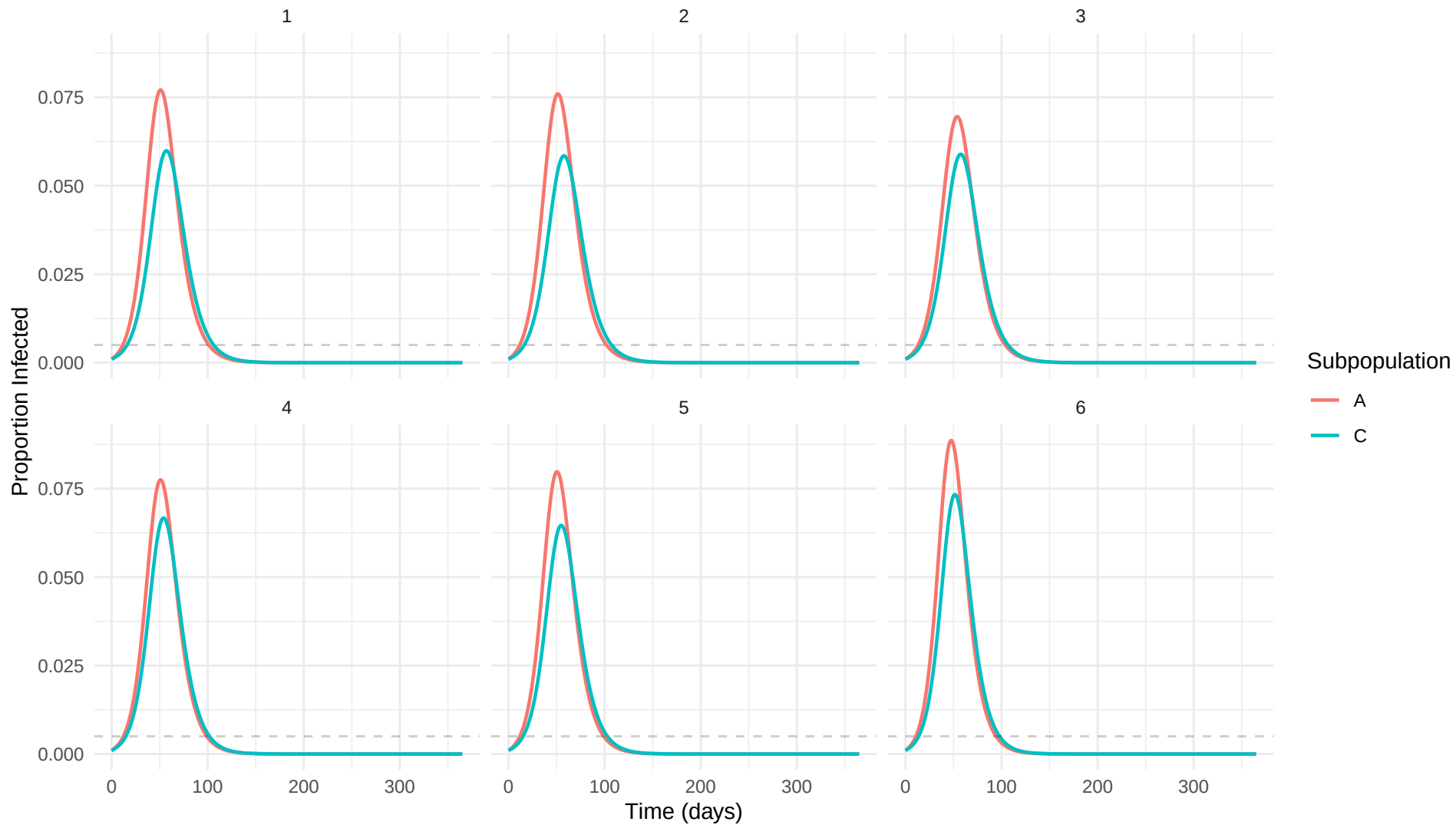
Infection curves: sar_0.2
