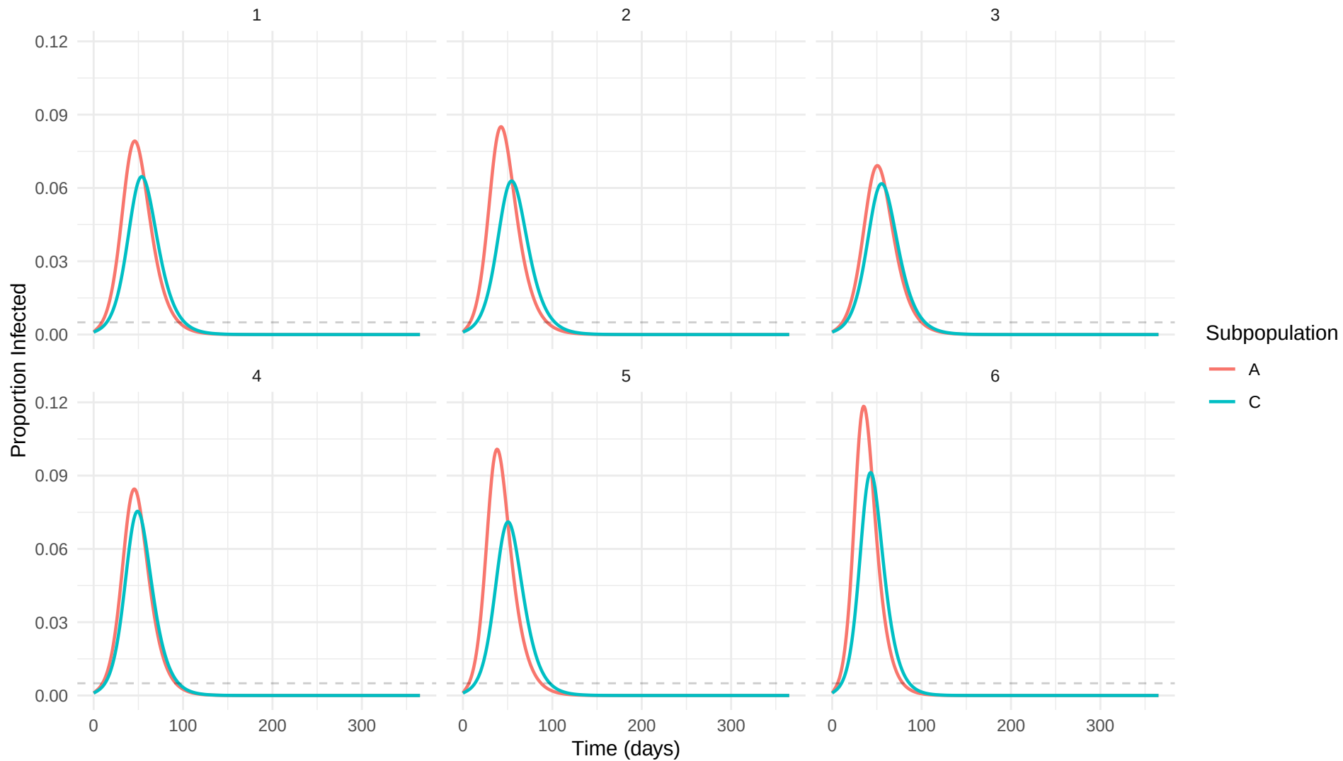
Infection curves: sar_0.6
