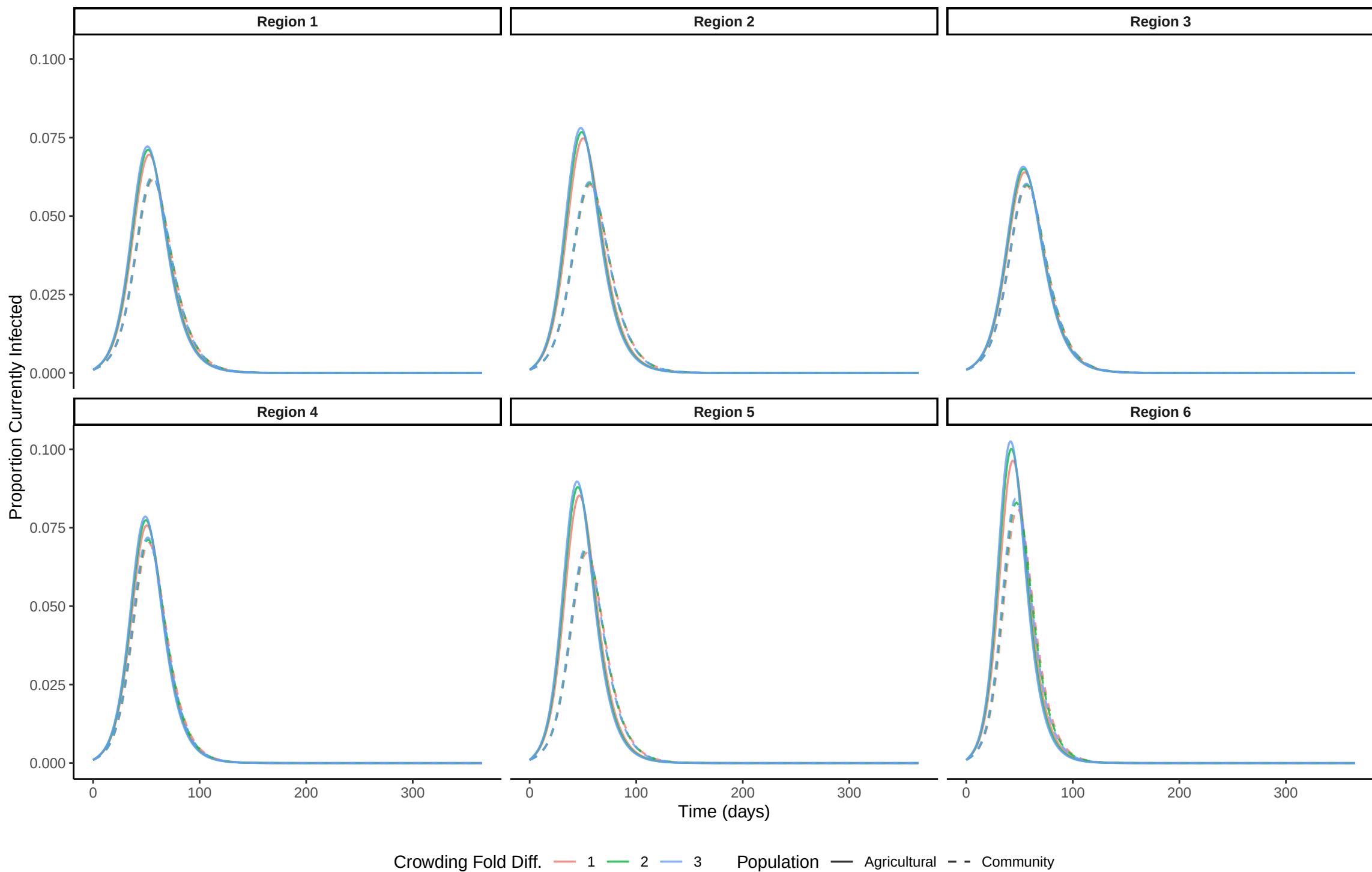
Epidemic Curves by Region – Sensitivity to Crowding Fold Diff.
