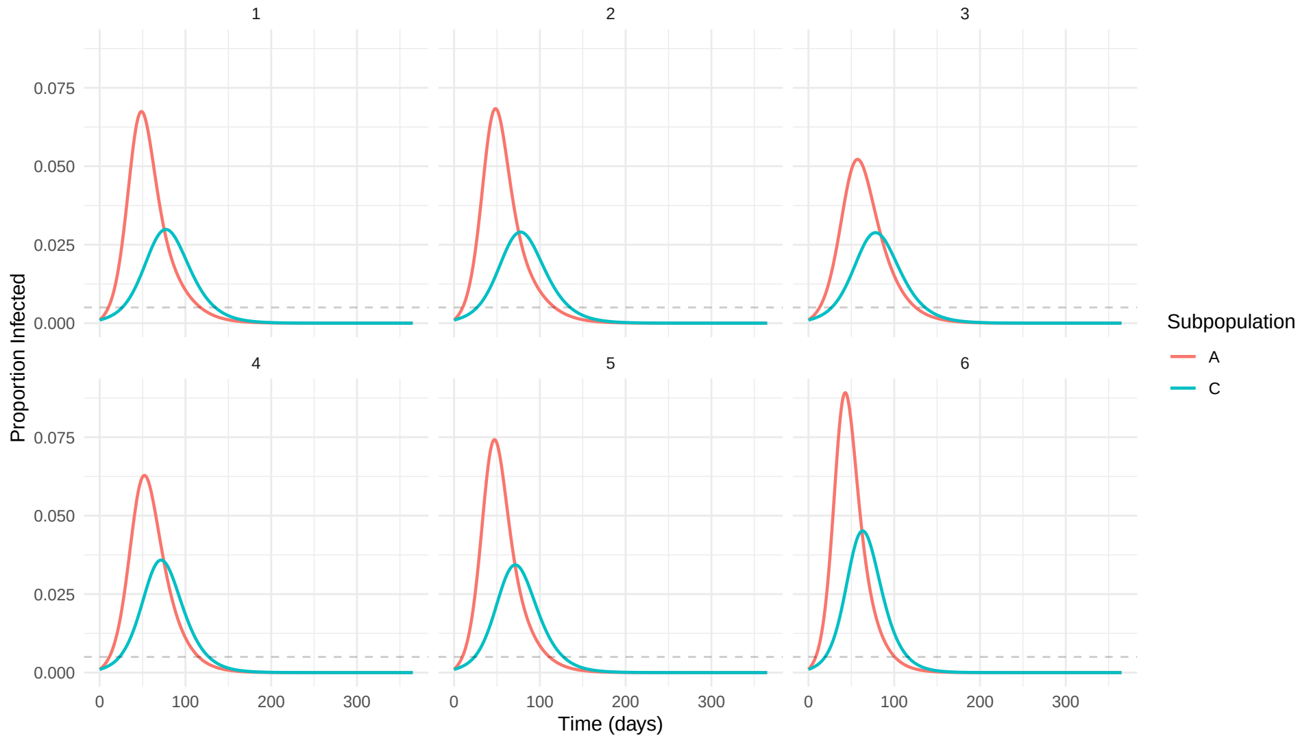
Infection curves: vax_C_0.6
