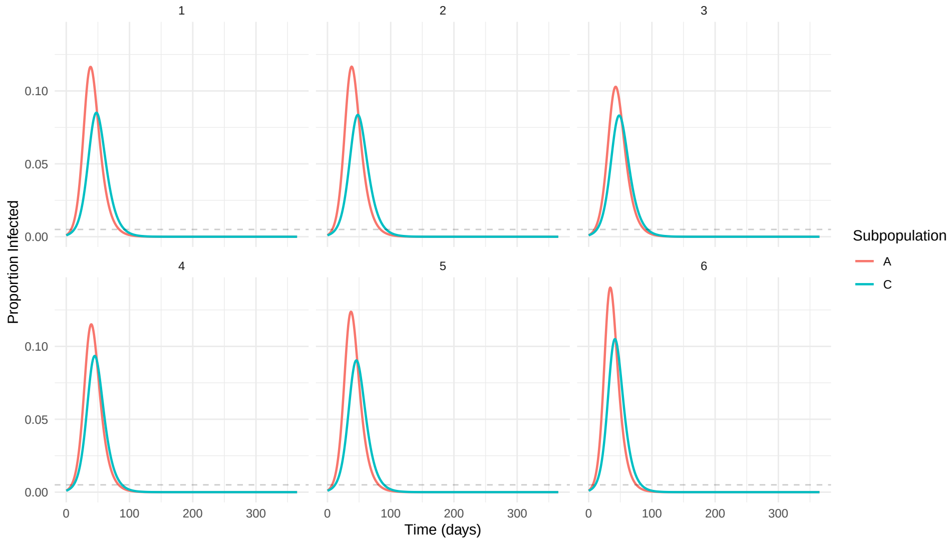
Infection curves: vax_eff_0.4
