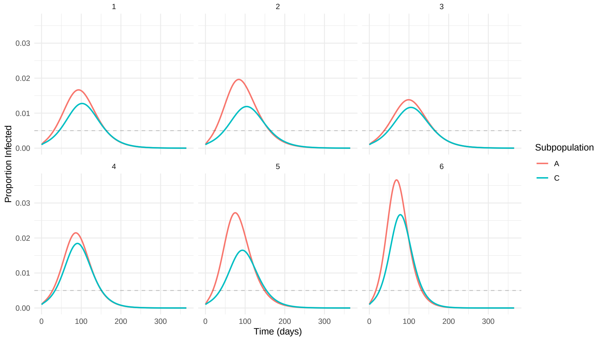
Infection curves: r0\_1.2
