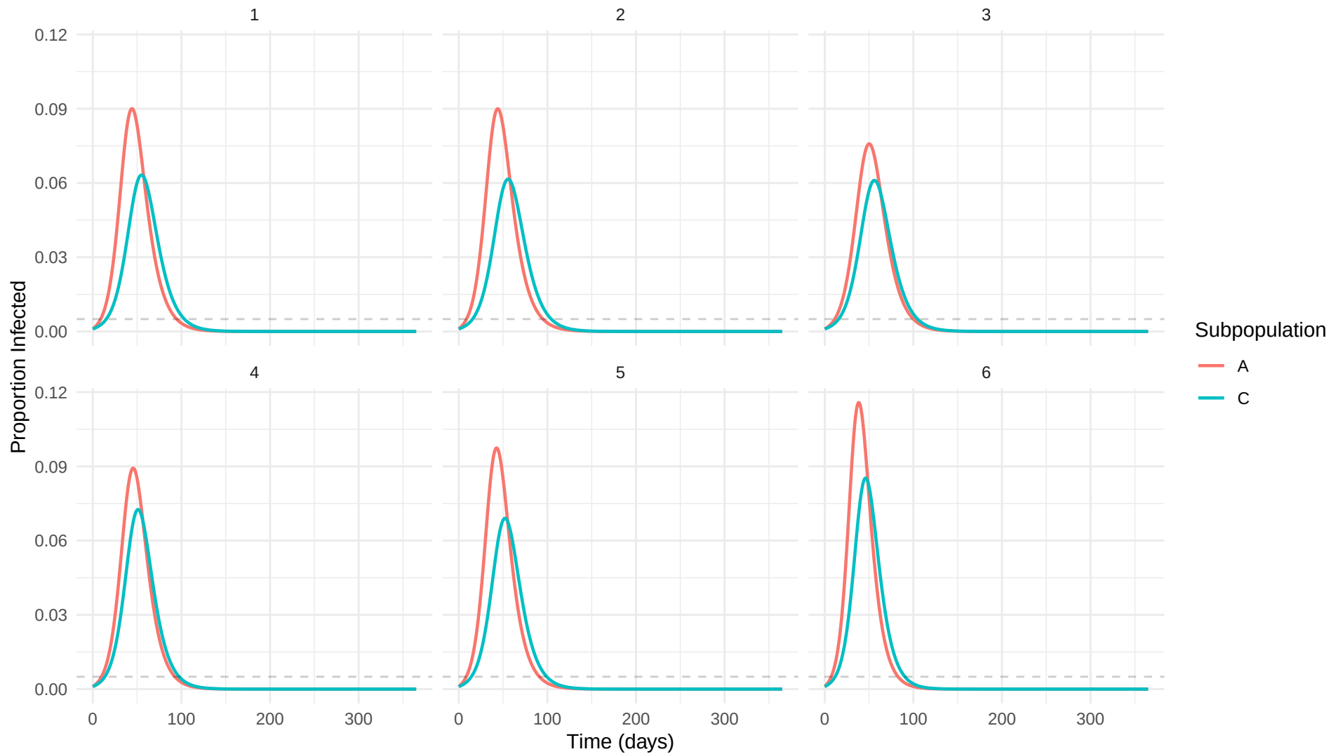
Infection curves: fold_3
