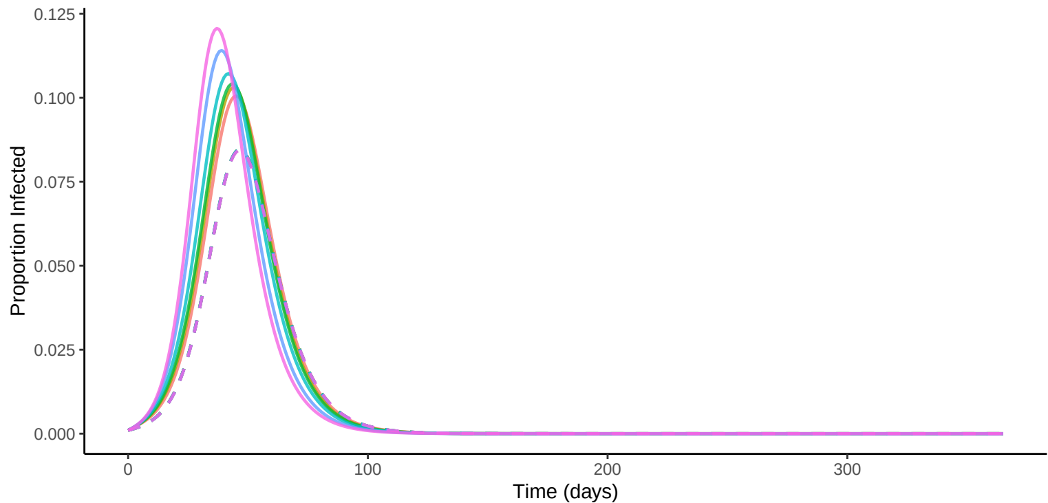
Epidemic Curves – Region 6
