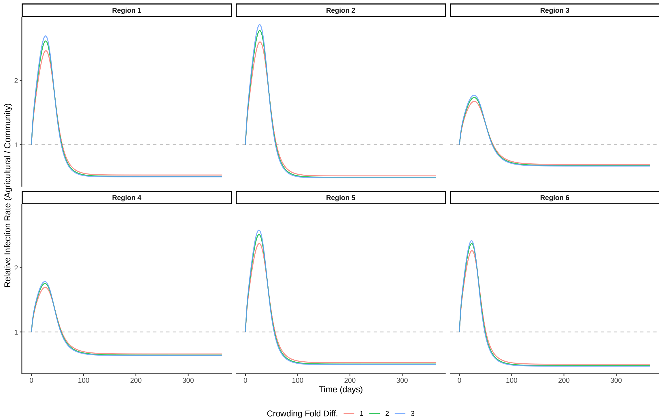
Relative Infection Rate by Region – Sensitivity to Crowding Fold Diff.
