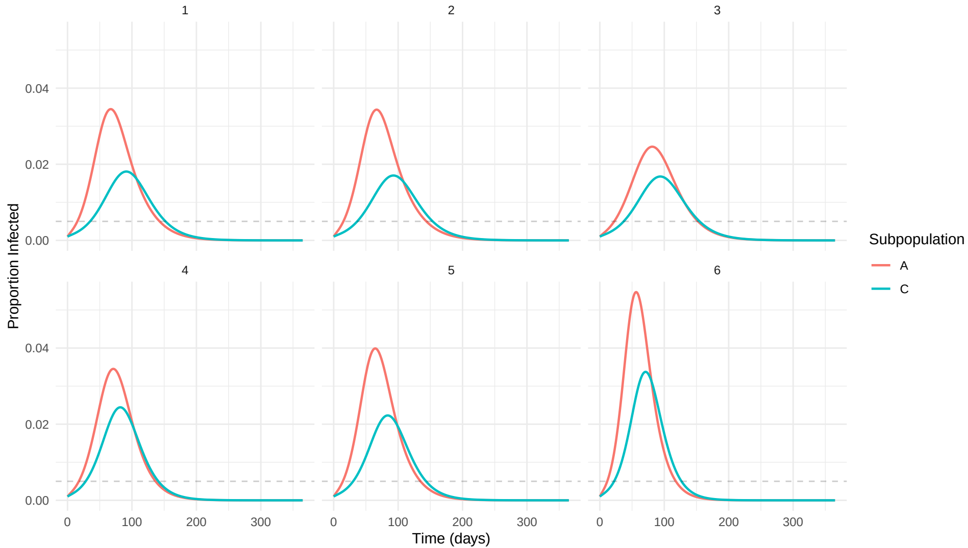
Infection curves: vax_C_0.4
