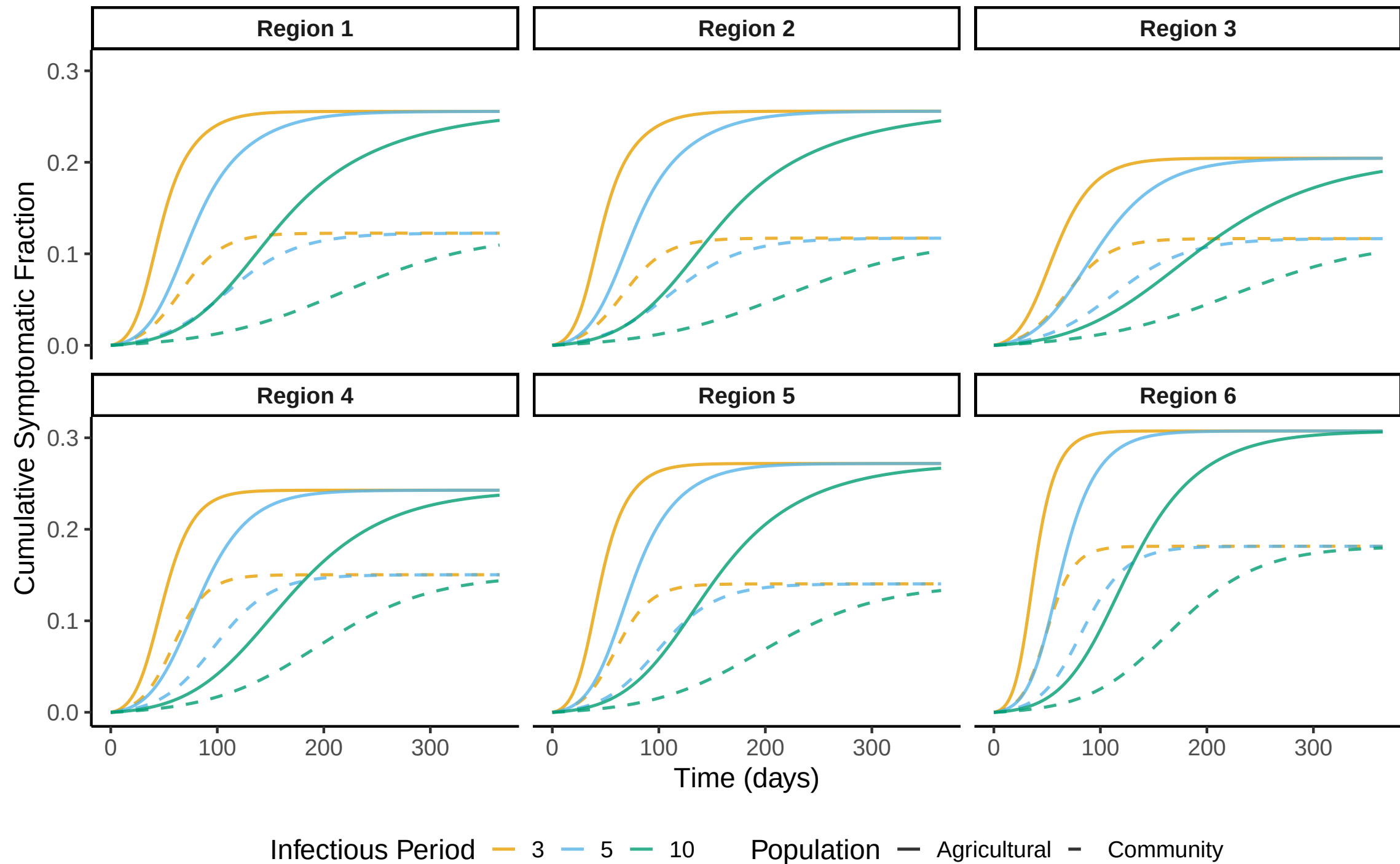
Cumulative Symptomatic Cases by Region – Sensitivity to Infectious Period
