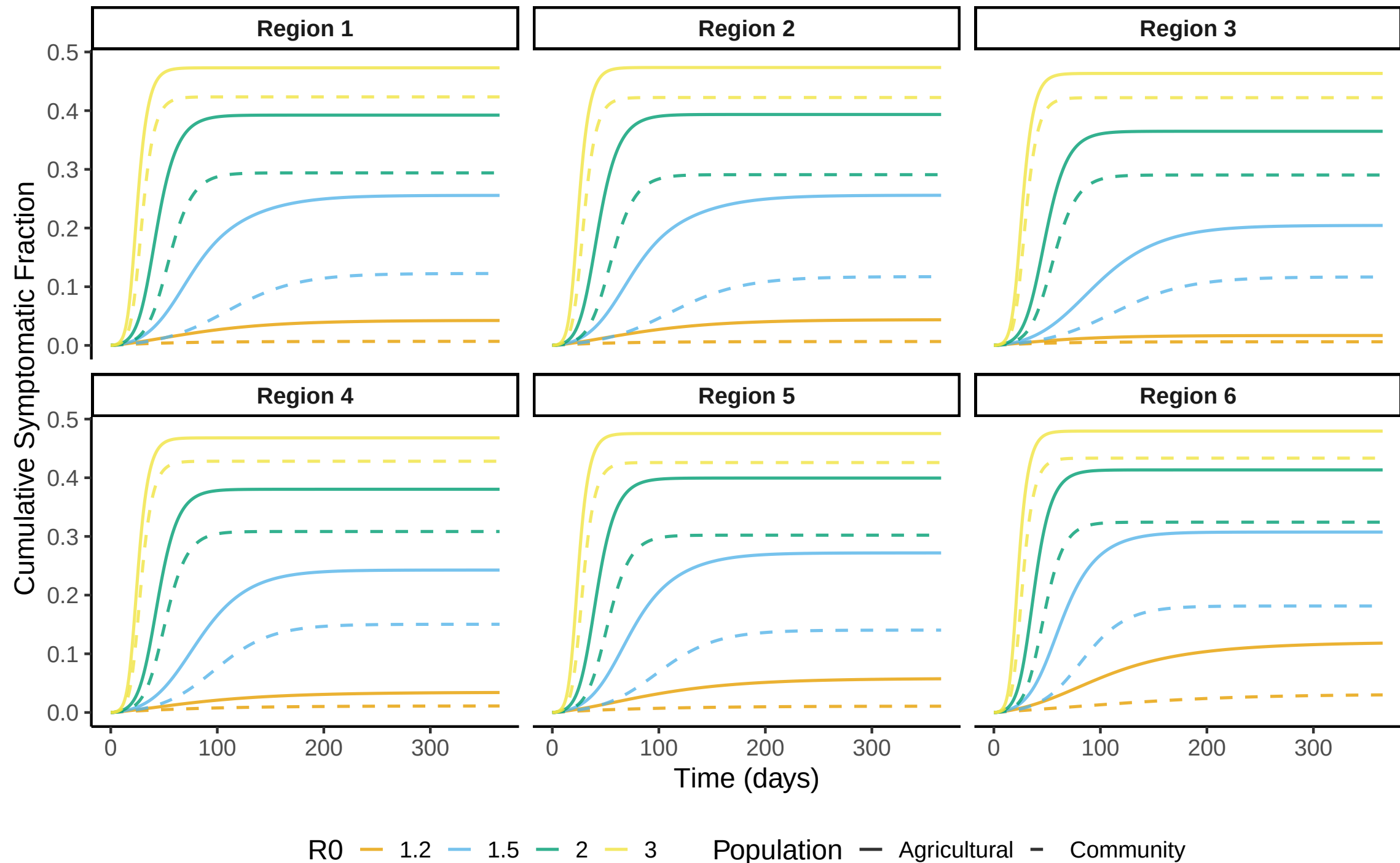
Cumulative Symptomatic Cases by Region – Sensitivity to R0
